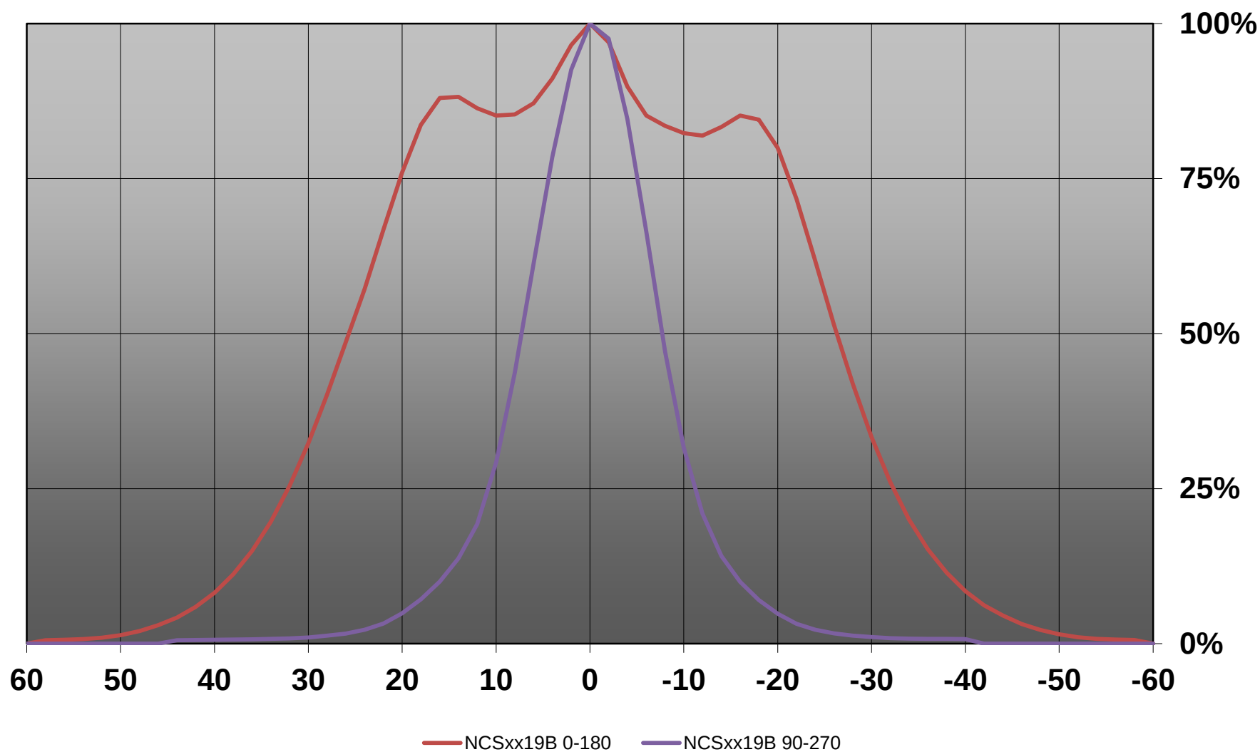
Relative intensity of C13529_VERONICA-O_(NCSxx19B)
