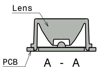
PCB suggestion
