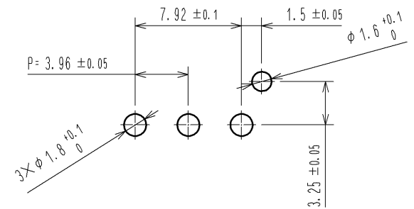
Recommended Pattern (free) (Recommended Board Thickness t=1.6mm)
