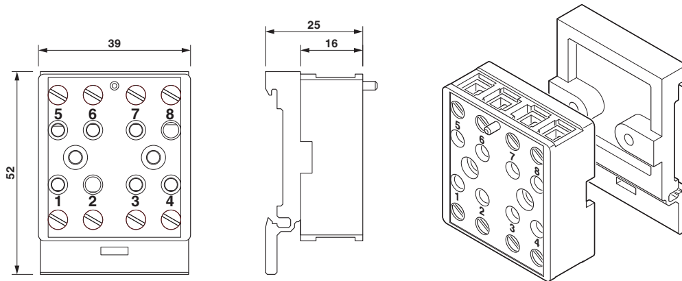
Dimensional drawing
