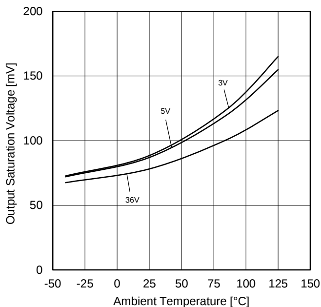
Figure 23. Output Saturation Voltage vs Ambient Temperature ( I_{\text{SINK}}=4\text{mA} )
