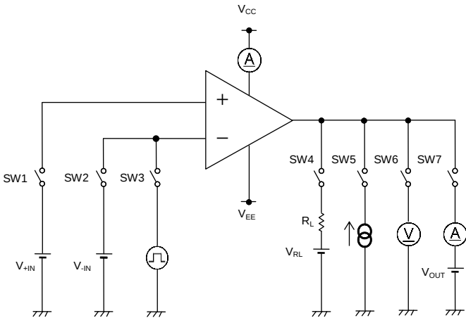
Figure 40. Test Circuit 2 (One Channel Only)
