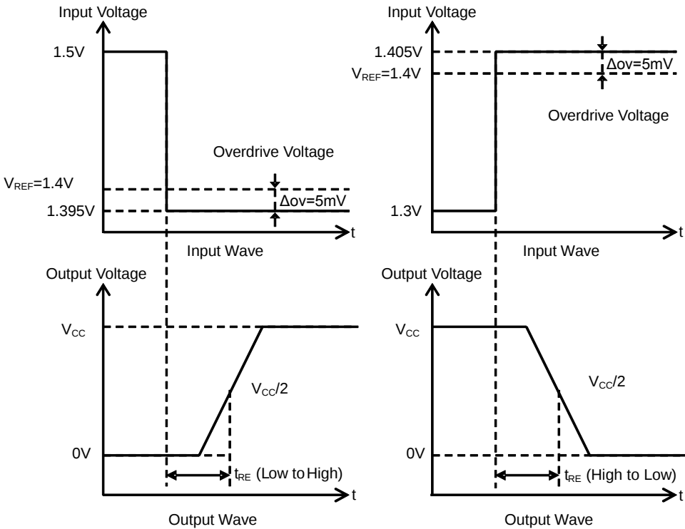
Figure 41. Response Time
