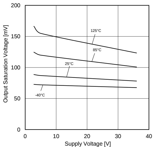
Figure 22. Output Saturation Voltage vs Supply Voltage ( I_{\text{SINK}}=4\text{mA} )
