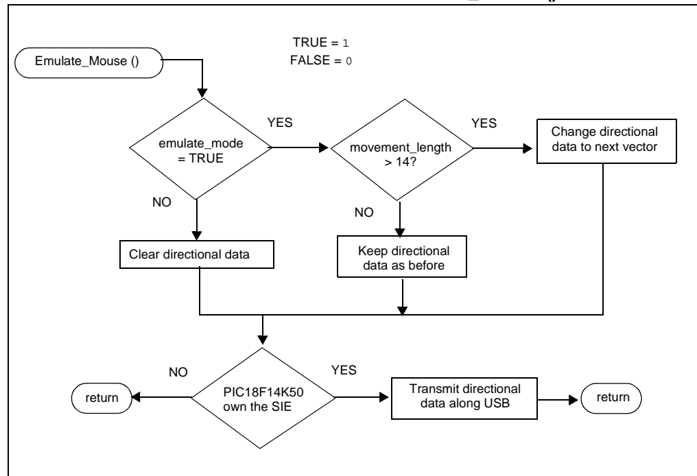
FIGURE 2-4: FLOWCHART FOR THE EMULATE_MOUSE()
