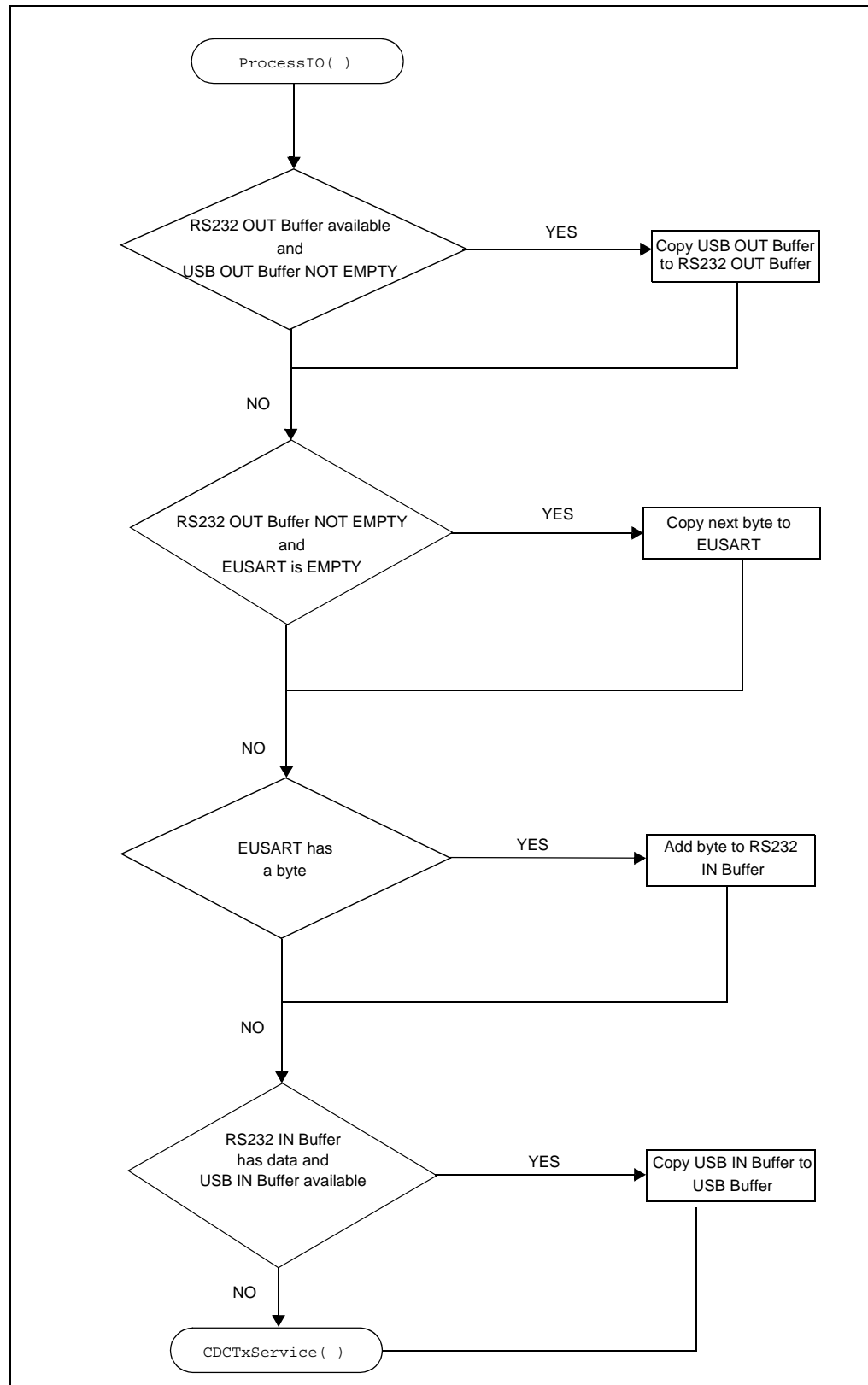
FIGURE 2-6: FLOWCHART FOR CDC SERIAL EMULATOR CODE
