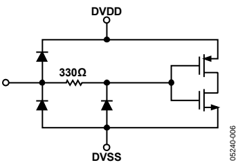
Figure 6. Digital Inputs
