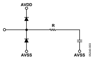
Figure 3. CCDIN_X
