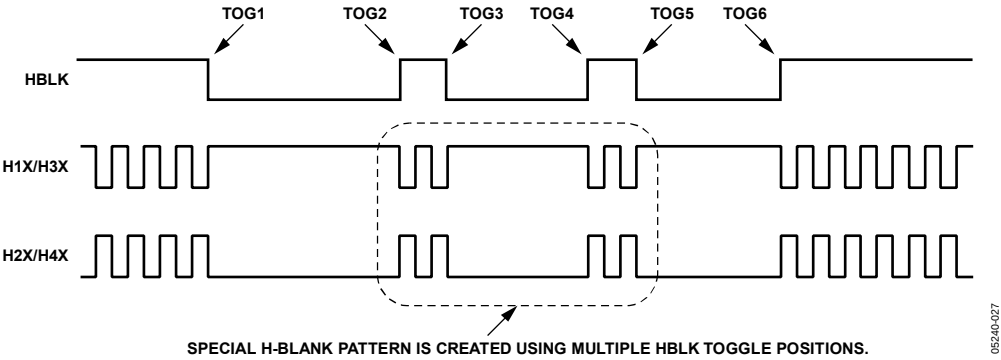
Figure 24. Generating Special HBLK Patterns
