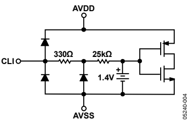
Figure 4. CLI_X
