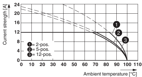
Type: MSTB 2,5/16-STF-5,08 with CC 2,5/16-GF-5,08 P26THR
