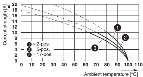
Type: MSTB 2,5/16-STF-5,08 with MDSTB 2,5/16-GF-5,08
