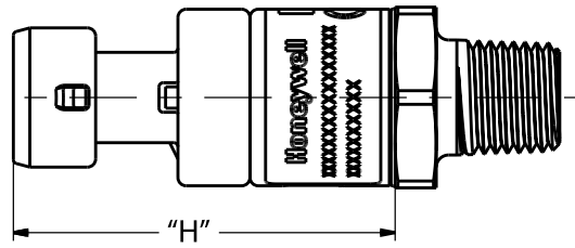
Figure 7. Connector Dimensions (For reference only: mm/[in].)
