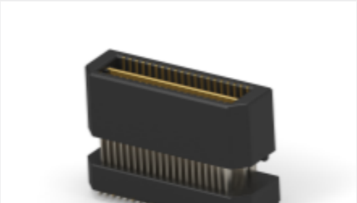
TE Part # 6-1658438-1 MSB0.80PL14ASY040FL,GP,10,-TR
