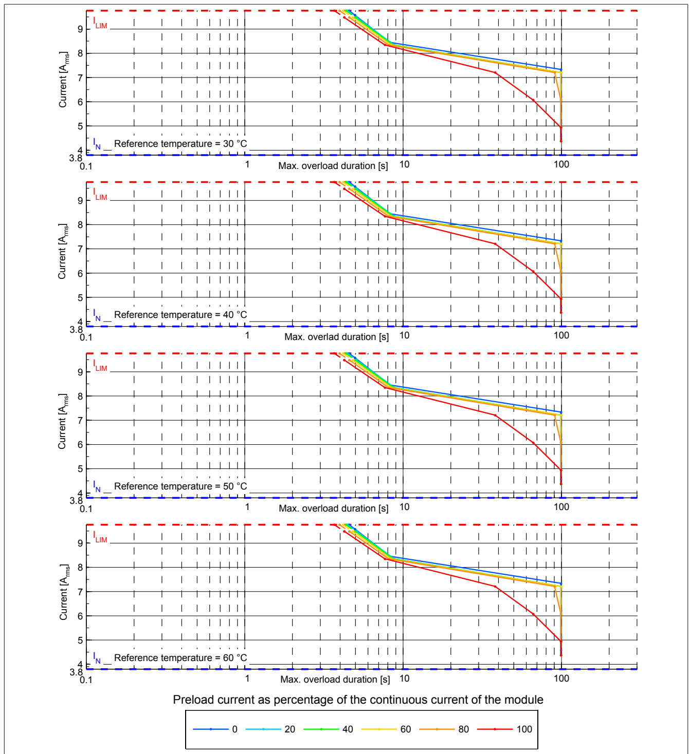
Figure 2: 8BVI0028HCSx.000-x_8BVI0028HCDx.000-x - Overload characteristics, overload response - ERROR+STOP
