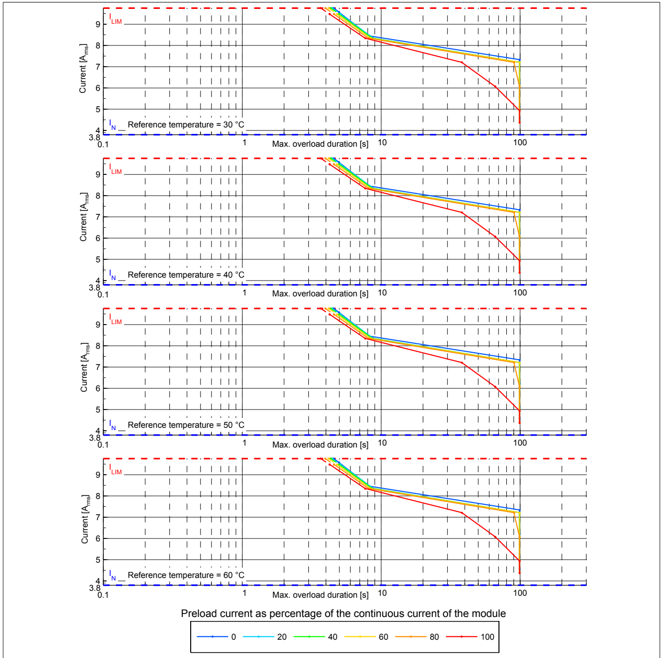
Figure 1: 8BVI0028HCSx.000-x_8BVI0028HCDx.000-x - Overload characteristics, overload response - WARNING
