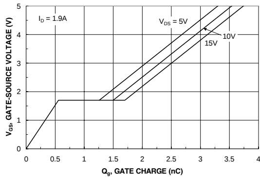
Figure 7. Gate-Charge Characteristics.
