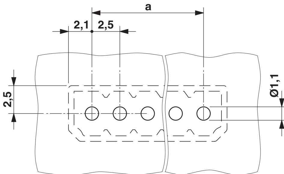
Dimensional drawing
