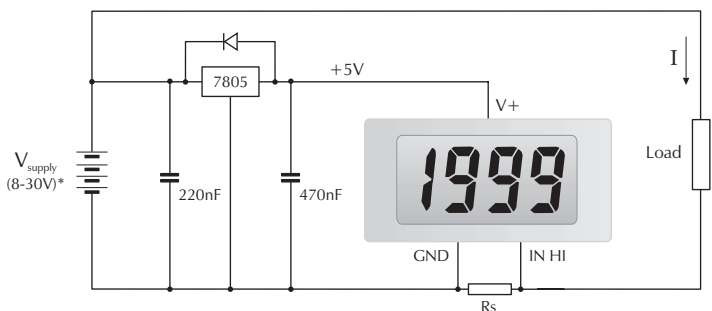
Measuring current.
