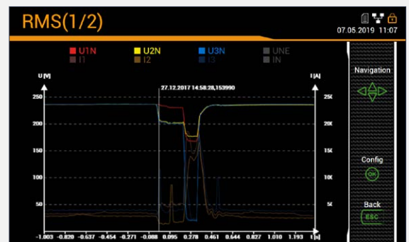
Voltage drop shown on local display
