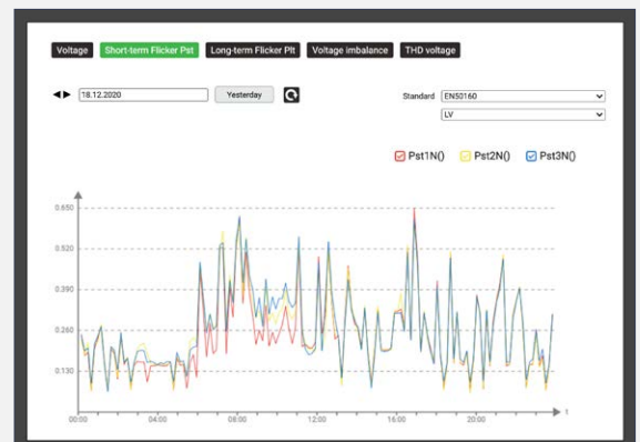
Progression of short-time flicker Pst during a day via the device website
