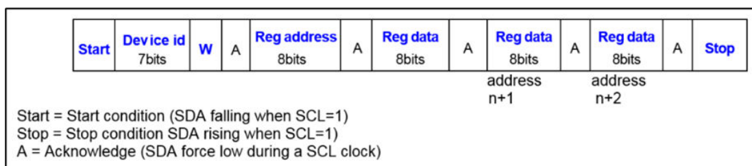
Figure 18. I 2 C write operation
