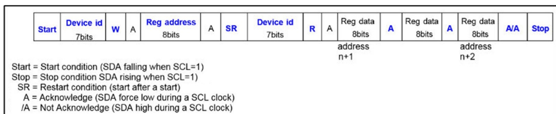
Figure 17. I 2 C read operation
