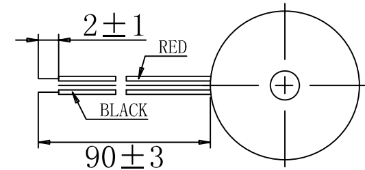
Dimensions Unit: mm Tolerance: ±0.5mm
