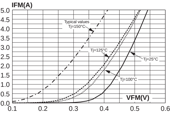
Fig. 9-2: Forward voltage drop versus forward current (maximum values, low level).
