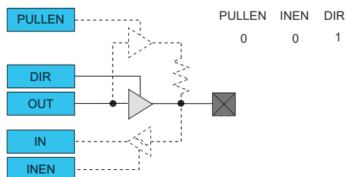
Figure 35-7. I/O Configuration - Totem-Pole Output with Enabled Input
