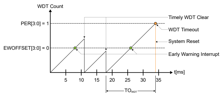
Figure 25-2. Normal-Mode Operation
