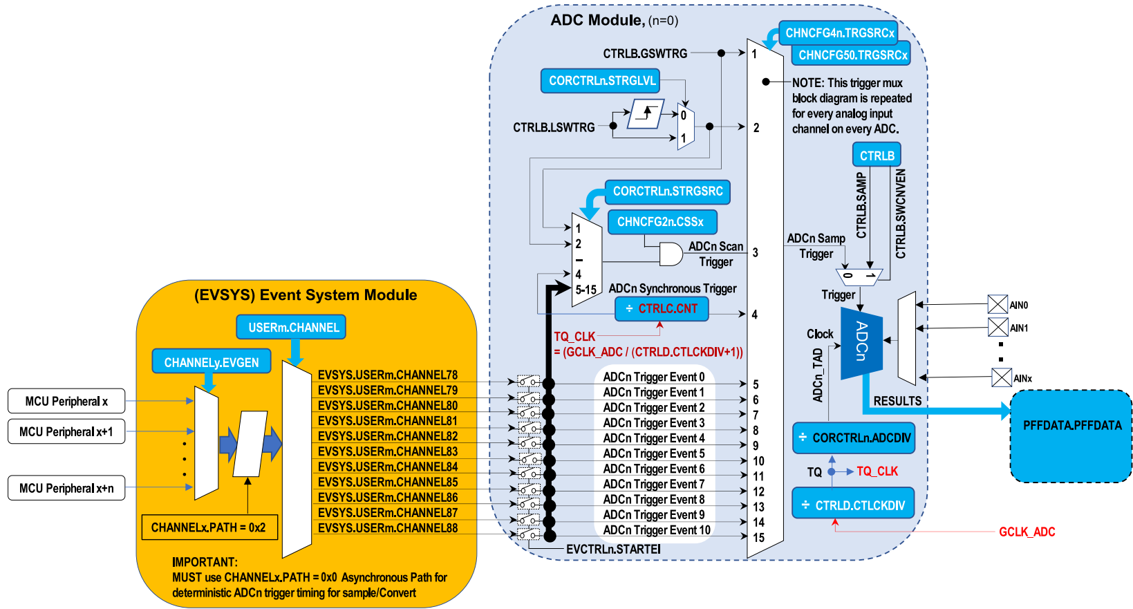
Figure 40-2. ADC Trigger Block Diagram
