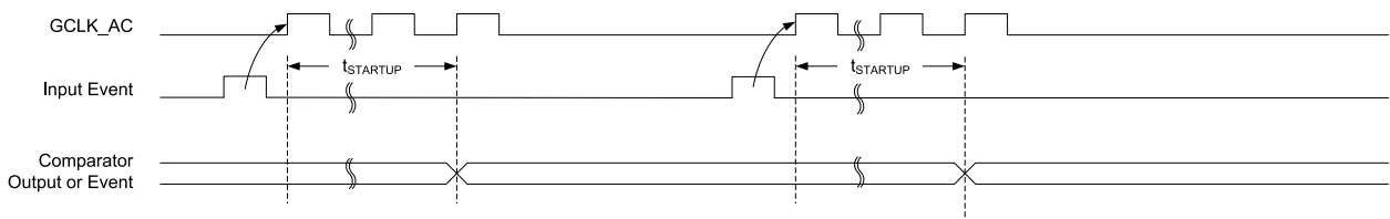
Figure 41-9. Single-Shot SleepWalking
