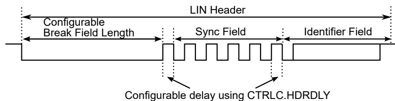
Figure 36-17. LIN Header Generation
