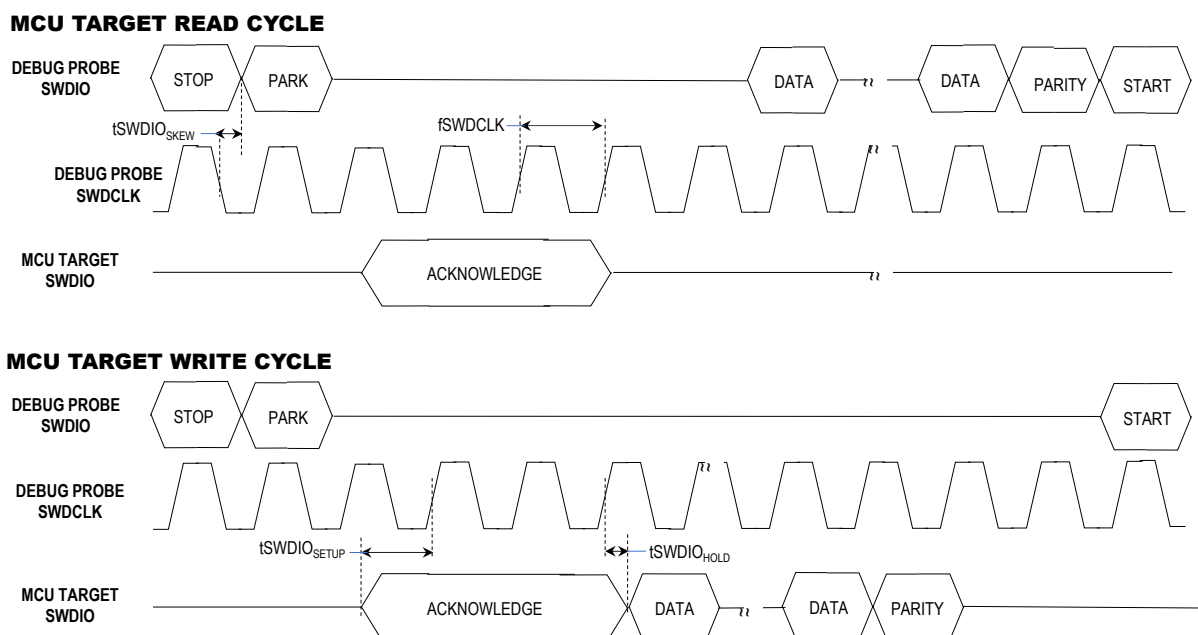
Figure 48-30. SWD 2-Wire Read/Write AC Timing Diagrams
