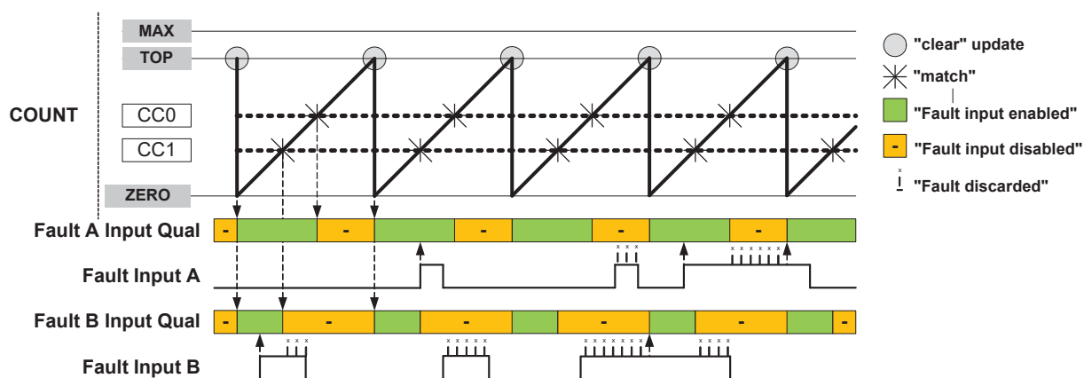
Figure 42-24. Fault Qualification in RAMP1 Operation
