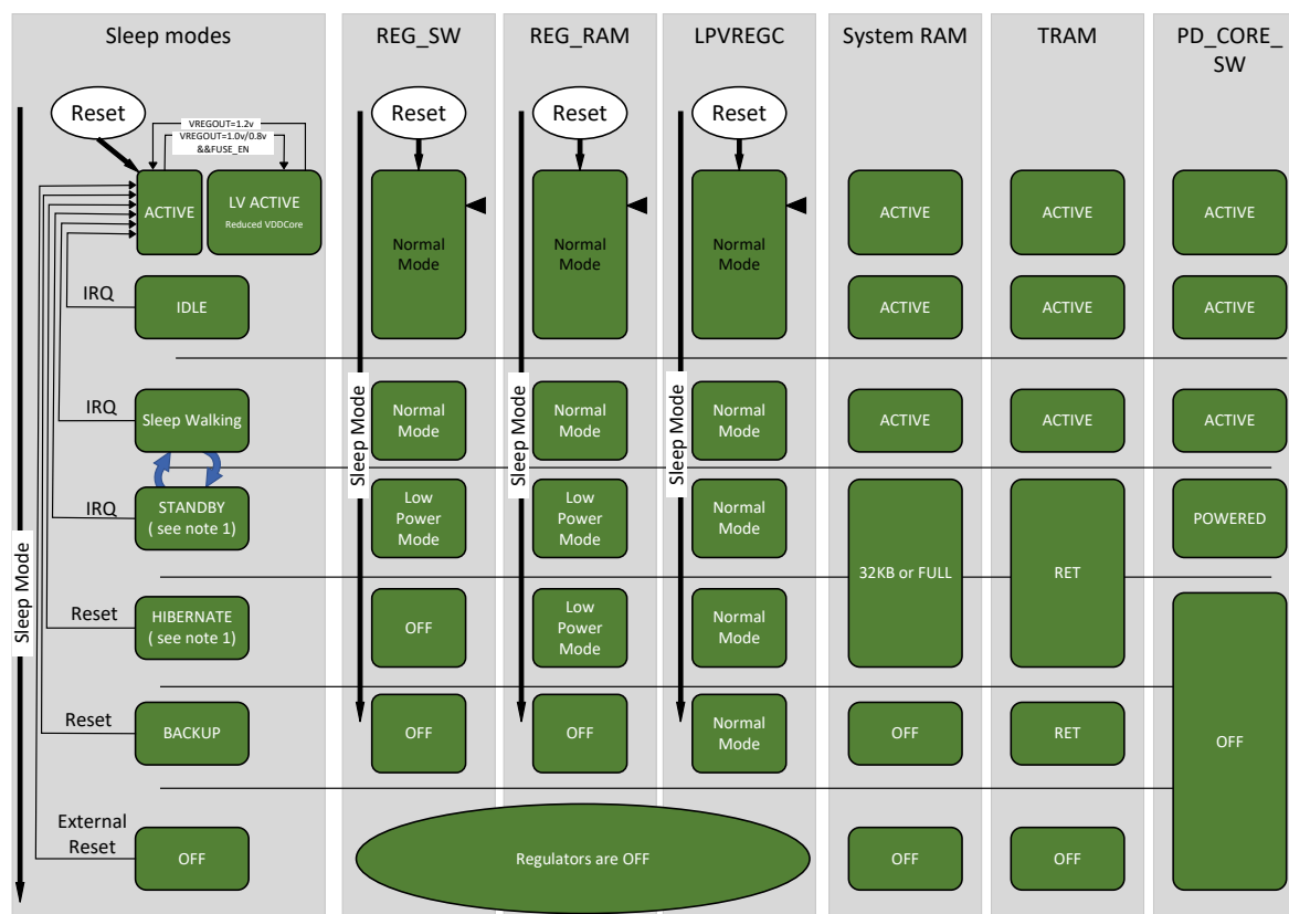
Figure 30-2. Operating Conditions and Sleepwalking
