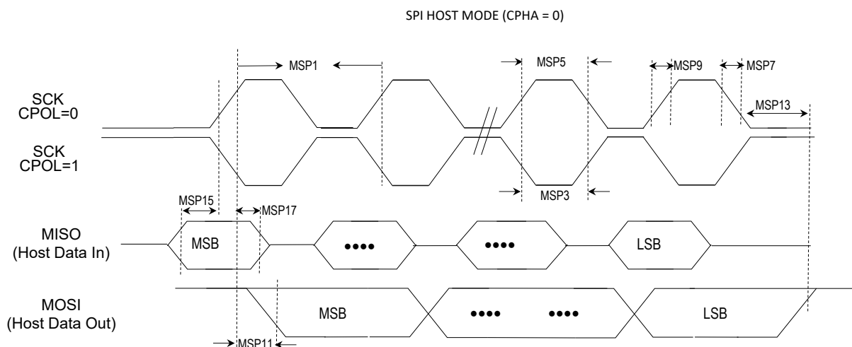
Figure 48-17. SPIx Host Module (CPHA = 0) Timing Diagrams
