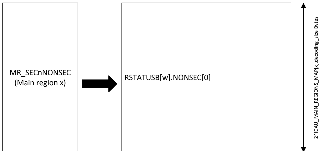
Figure 14-3. SECNONSEC_B Layout
