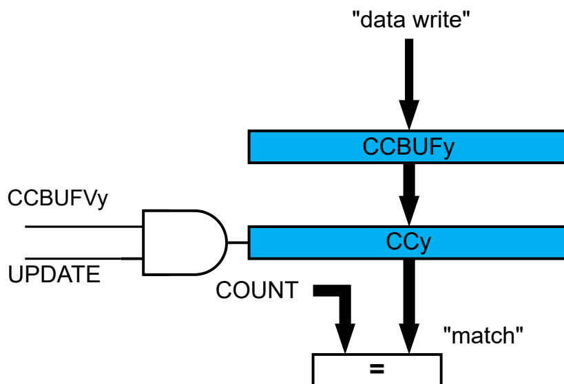
Figure 42-9. Compare Channel Double Buffering
