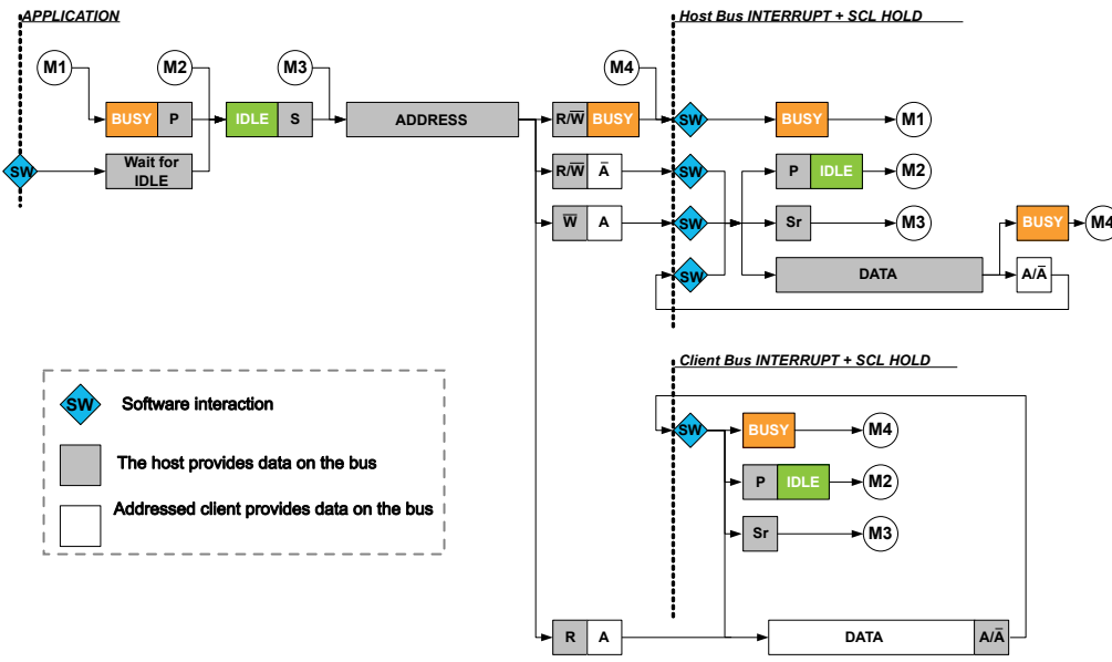
Figure 36-46. I 2 C Host Behavioral Diagram (SCLSM = 1)
