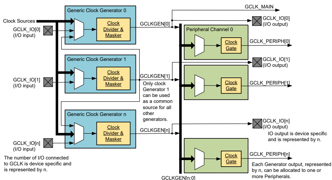
Figure 22-2. Generic Clock Controller Detailed Block Diagram
