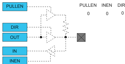
Figure 35-9. I/O Configuration - Reset or Analog I/O: Digital Output, Input and Pull Disabled
