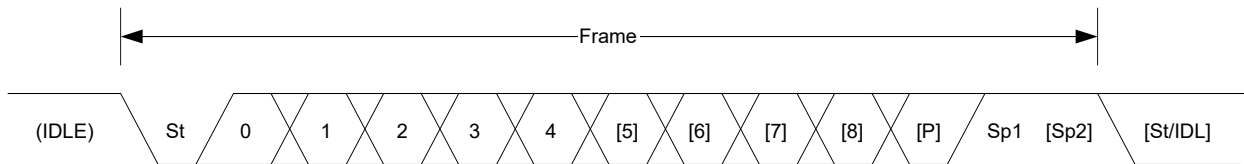
Figure 36-8. Frame Formats
