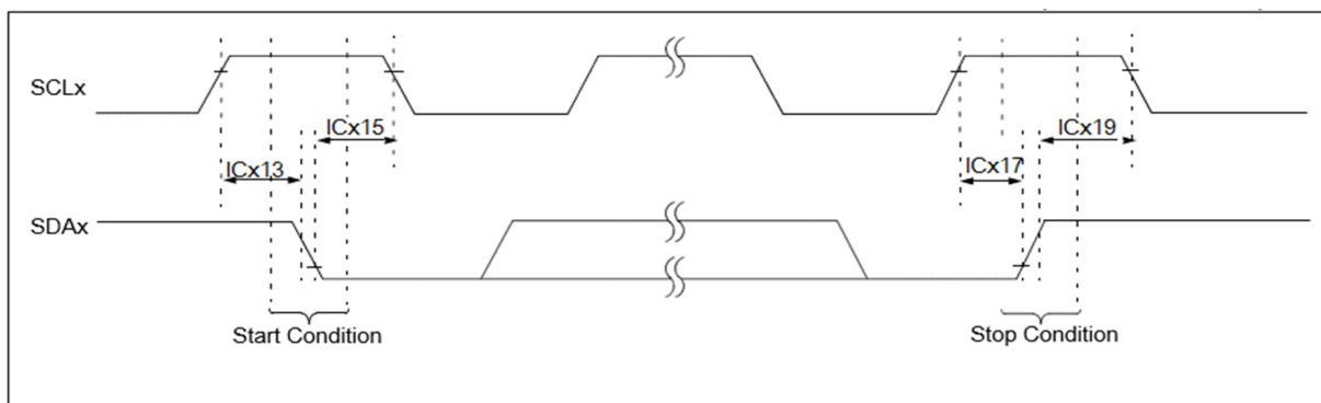
Figure 48-22. I 2 C Bus Data Host Mode AC Timing Diagrams
