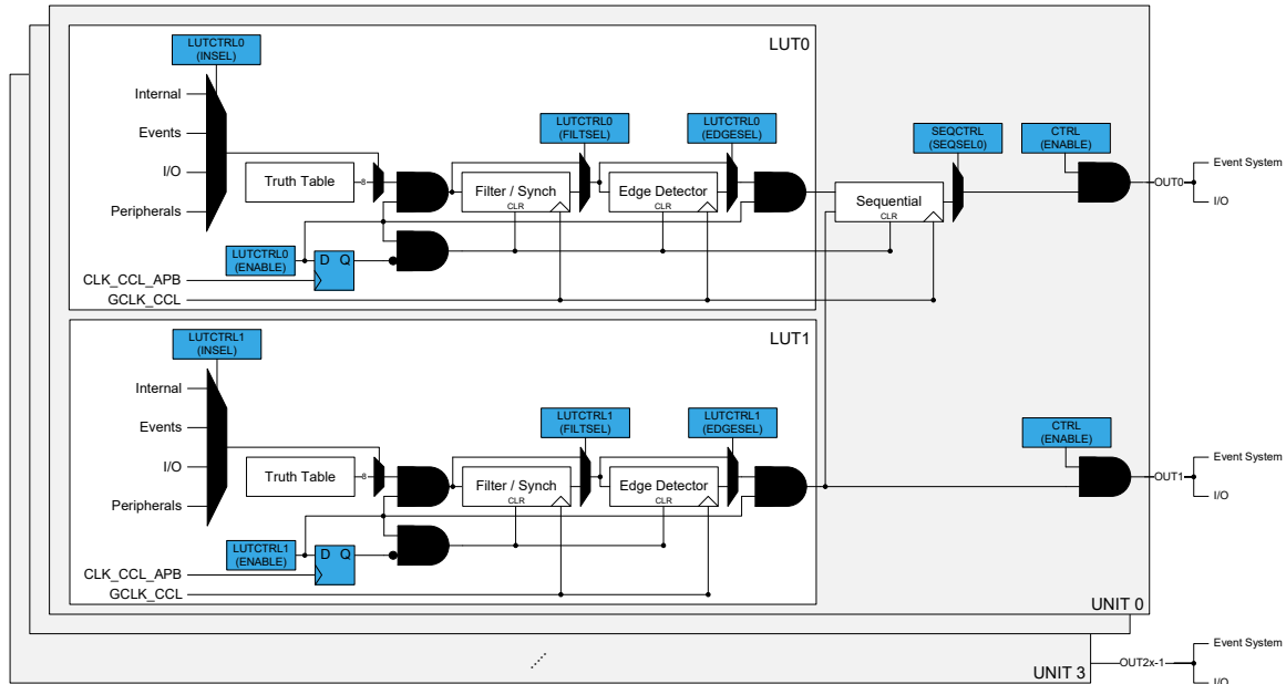
Figure 39-1. Configurable Custom Logic
