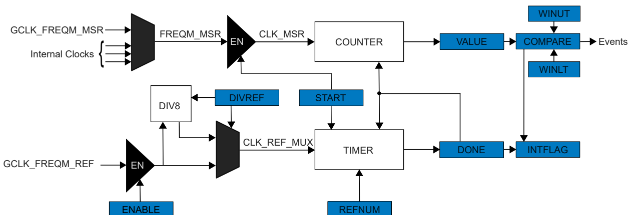
Figure 26-1. FREQM Block Diagram
