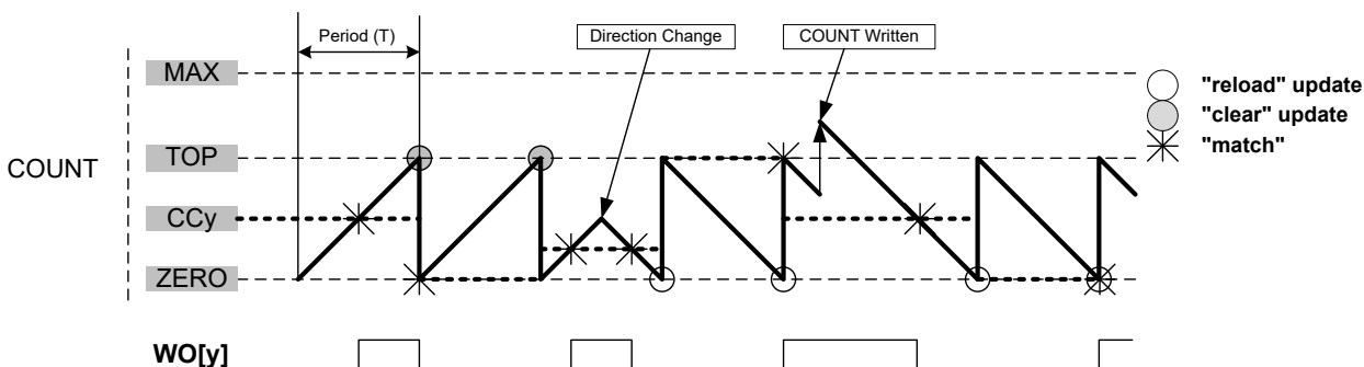
Figure 42-3. Normal Frequency Operation
