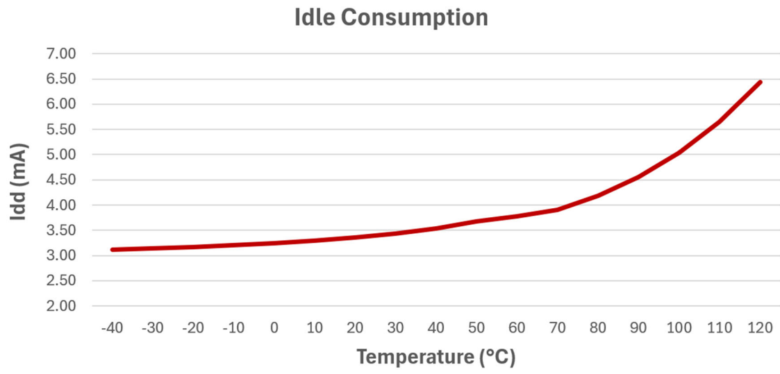
Figure 49-2. Power Consumption over Temperature in Idle Mode (Typical values for guidance only, not characterized over Process/voltage)
