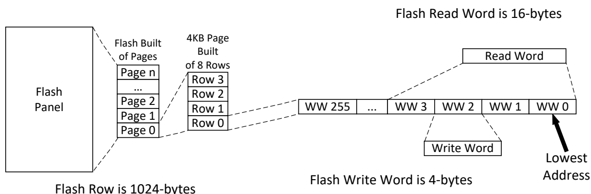
Figure 33-1. Flash Module Construction
