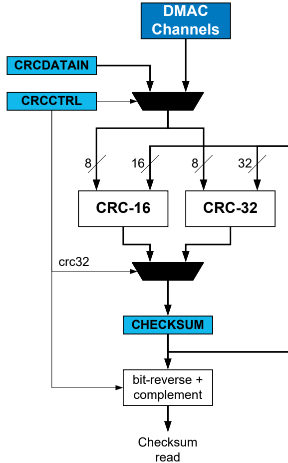
Figure 28-15. CRC Generator Block Diagram
