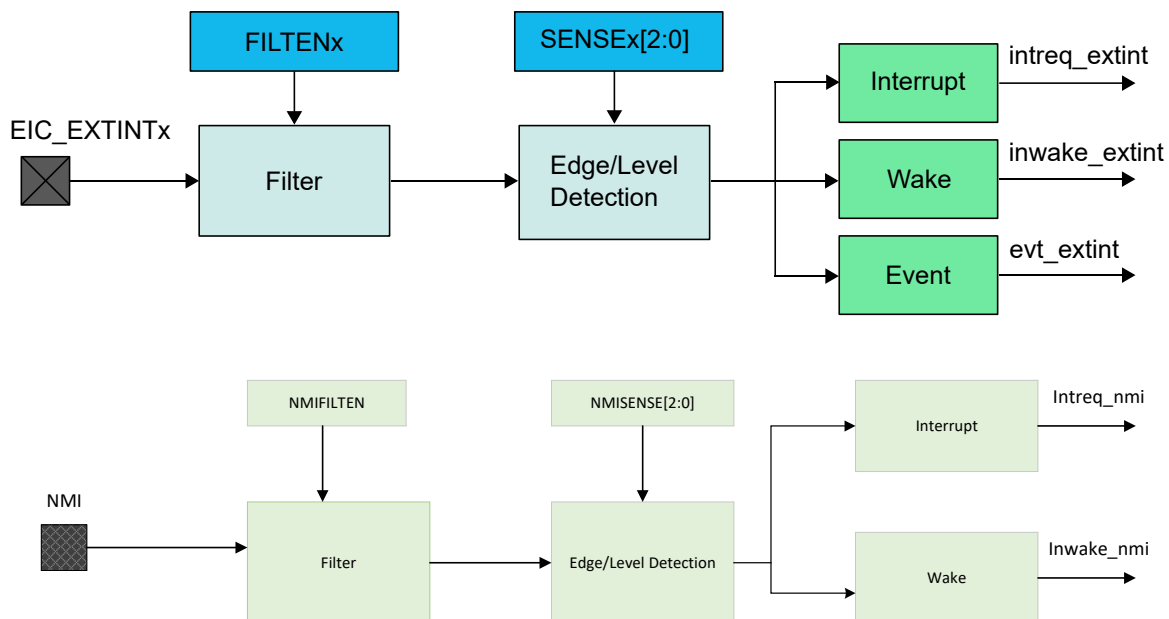
Figure 32-1. EIC Block Diagram
