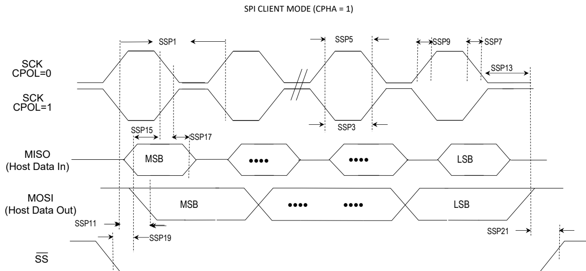
Figure 49-10. SPIx Client Module (CPHA = 1) Timing Diagrams
