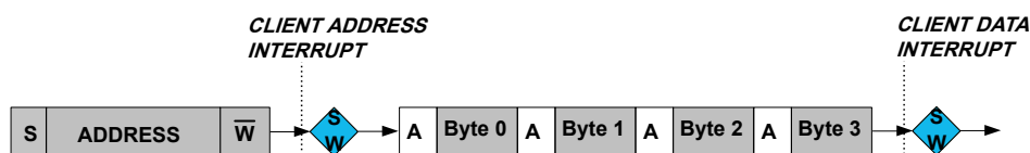
Figure 36-56. 32-bit Extension Client Operation
