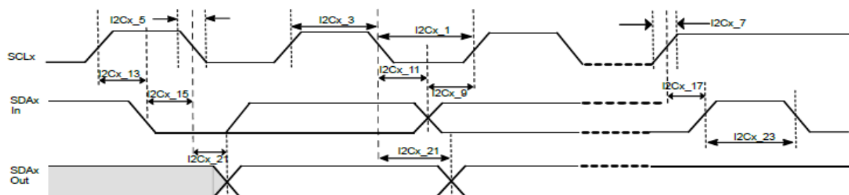
Figure 48-24. I 2 C Bus Data Client Mode AC Timing Diagrams
