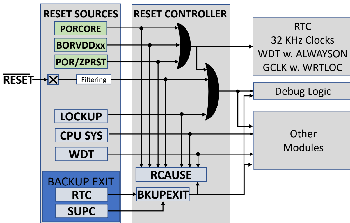
Figure 31-1. Reset Controller Block Diagram
