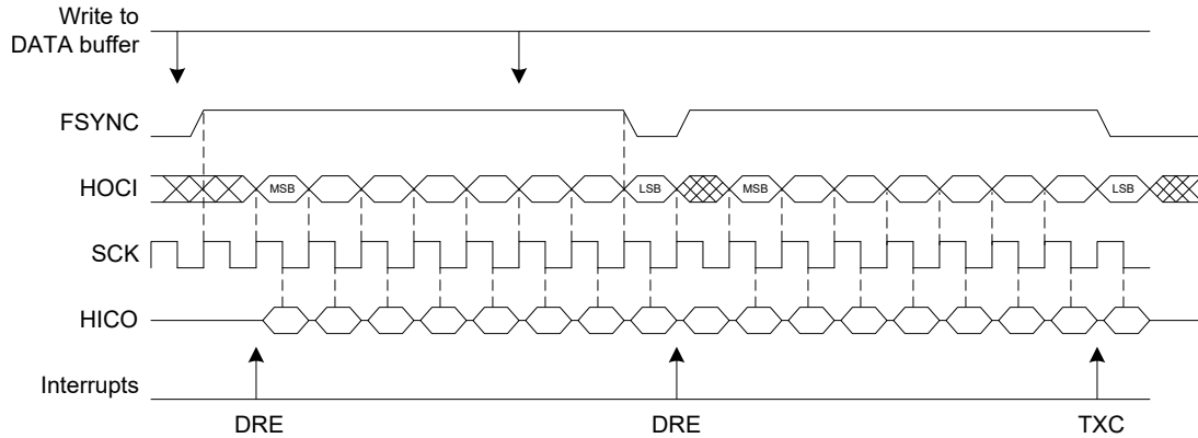
Figure 36-36. FMODE = HOST, FSPOL = HIGH, FSLEN = LEVEL, FSES = 0
