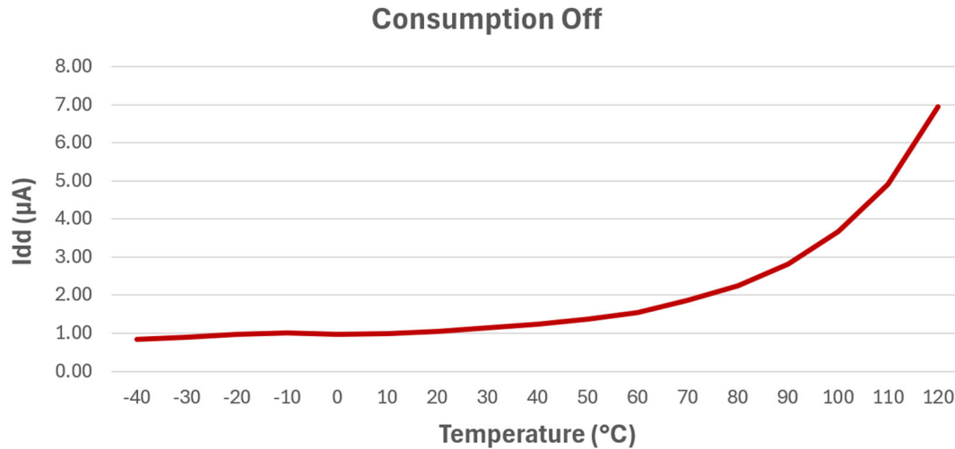
Figure 49-6. Power Consumption over Temperature in Off Mode (Typical values for guidance only, not tested)
