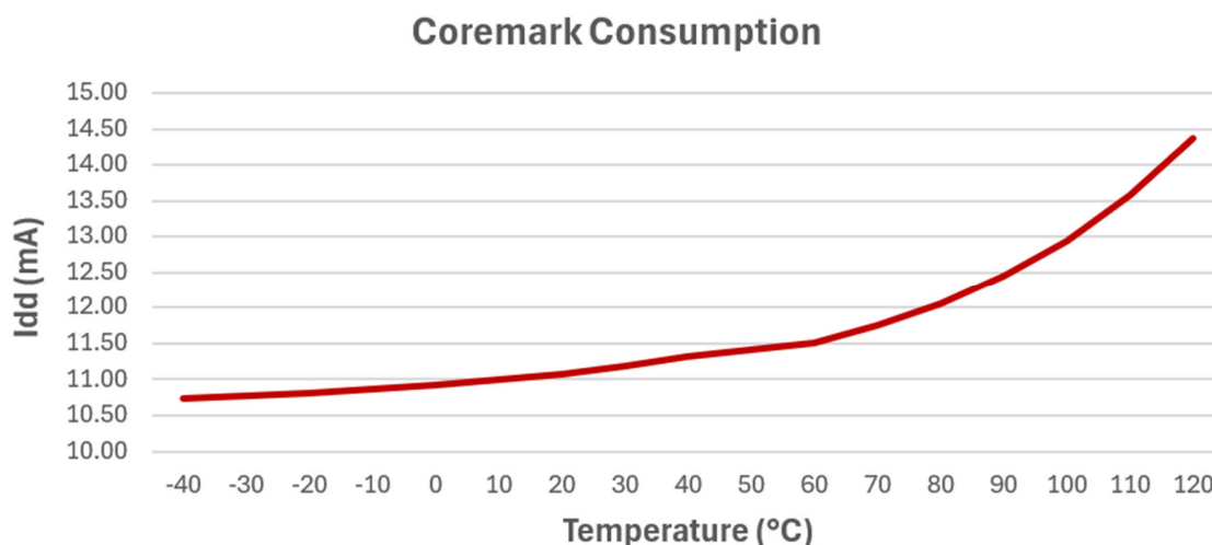
Figure 48-1. Power Consumption over Temperature in Active Mode (Typical values for guidance only, not tested)
