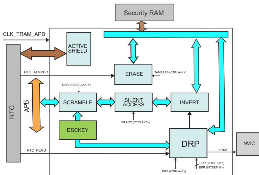
Figure 43-1. Block Diagram
