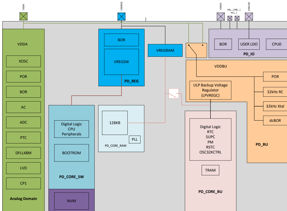
Figure 29-1. Supply Controller Block Diagram
