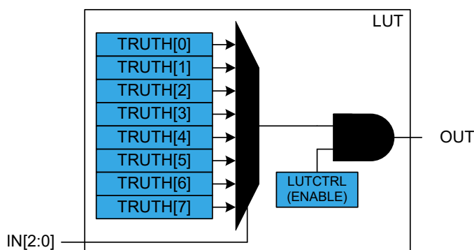
Figure 39-2. Truth Table Output Value Selection
