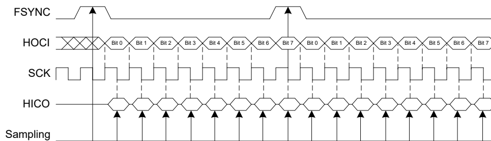
Figure 36-39. FMODE = CLIENT, FSPOL = HIGH, FSLEN = STROBE, FSES = 0
