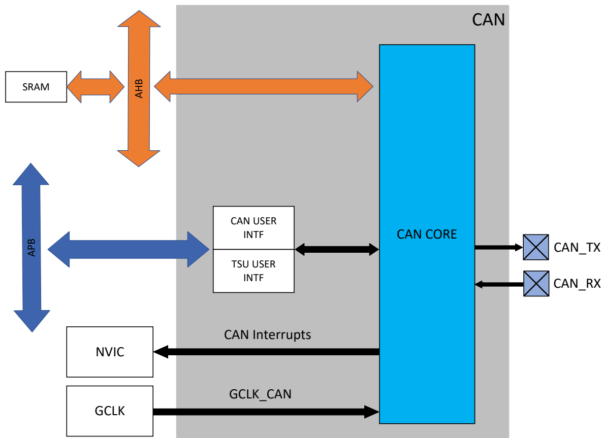
Figure 37-1. Block Diagram
