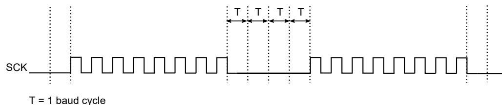
Figure 36-32. Four Cycle Inter-Character Spacing Example
