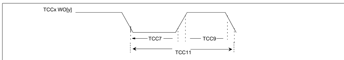
Figure 48-28. TCCx Timer Compare Fault Output Module AC Timing Diagrams
