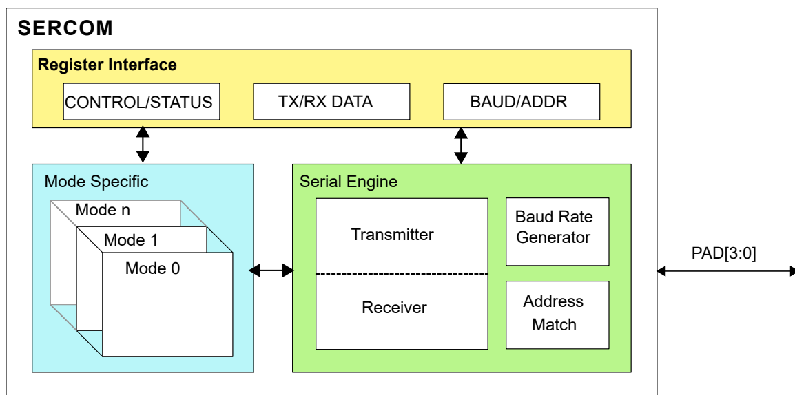
Figure 36-1. SERCOM Block Diagram
