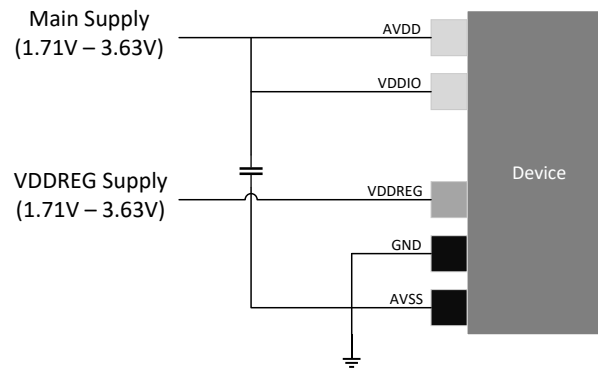
Figure 8-3. Power Supply for Dual Voltage Mode
