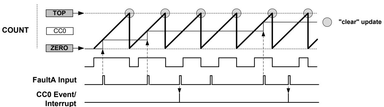
Figure 42-29. Capture Action "CAPTMAX"
