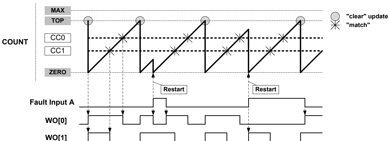
Figure 42-28. Waveform Generation in RAMP2 Operation with Restart Action
