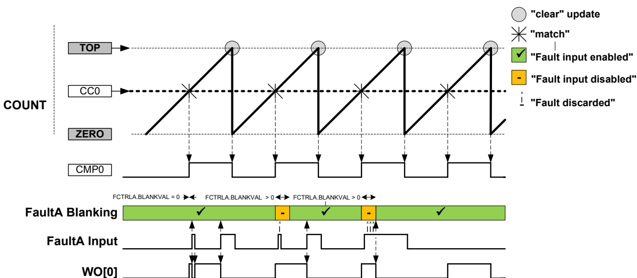
Figure 42-23. Fault Blanking in RAMP1 Operation with Inverted Polarity
