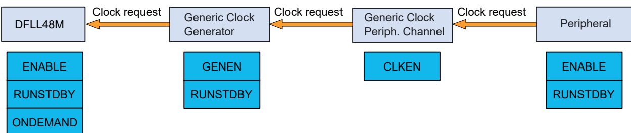
Figure 20-3. Clock Request Routing
