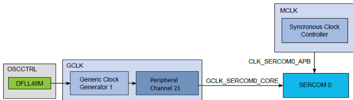
Figure 20-2. Example of SERCOM clock
