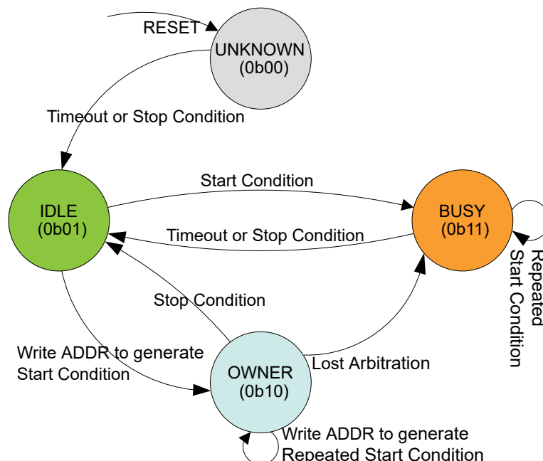
Figure 36-44. Bus State Diagram
