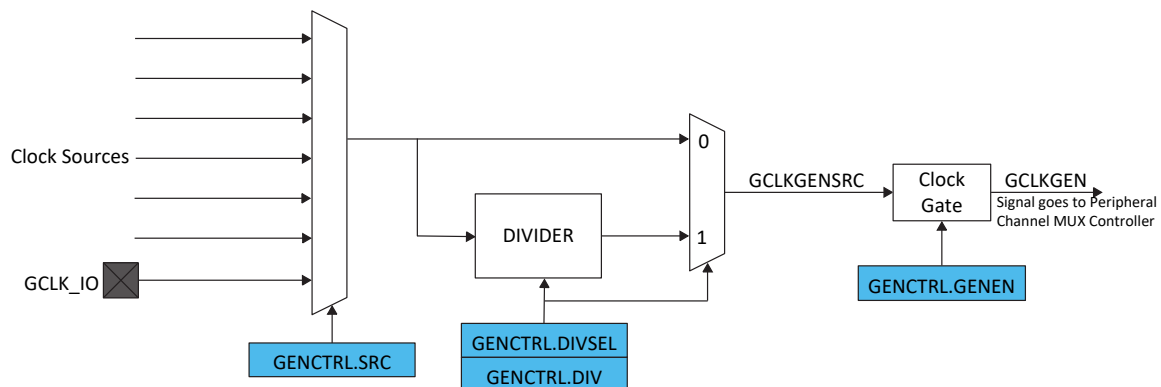
Figure 22-3. Generic Clock Generator
