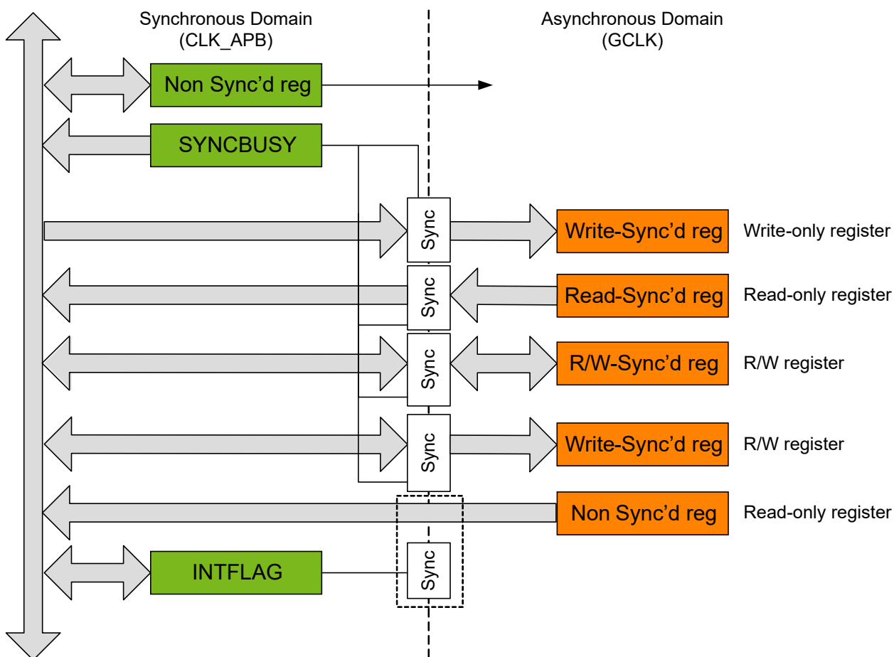
Figure 10-1. Register Synchronization Overview
