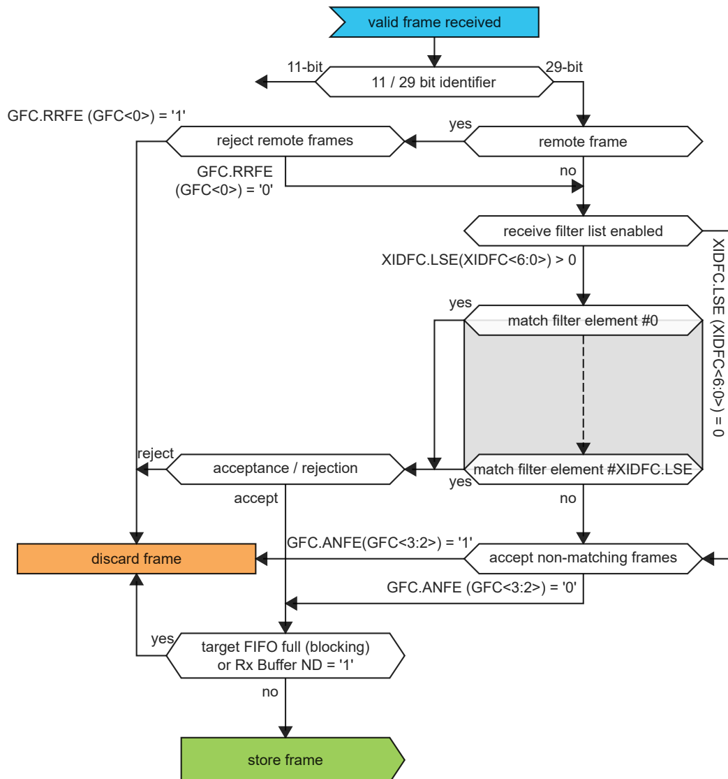
Figure 37-6. Extended Message ID Filtering
