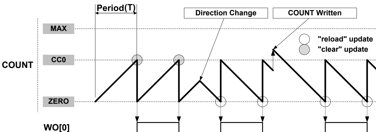
Figure 42-4. Match Frequency Operation
