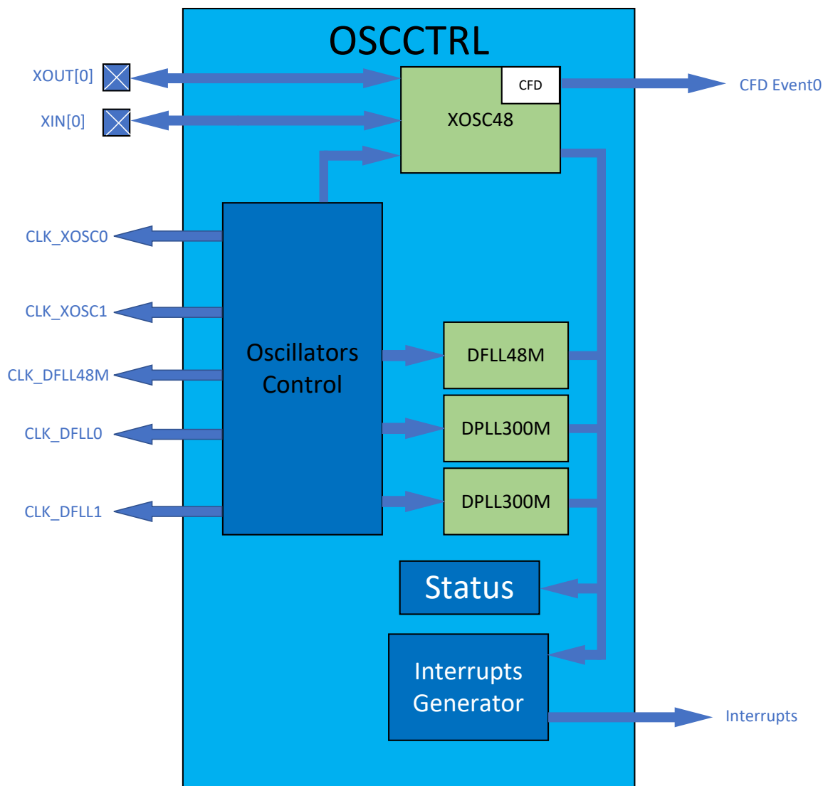
Figure 21-1. OSCCTRL Block Diagram
