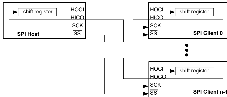
Figure 36-30. Multiple Clients in Series
