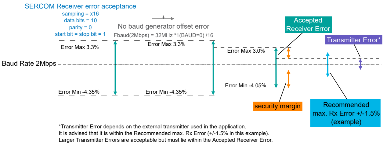
Figure 36-12. USART Rx Error Calculation Example
