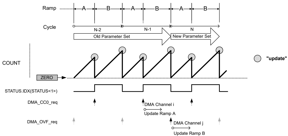
Figure 42-35. DMA Triggers in RAMP2 Operation and Circular Buffer Enabled
