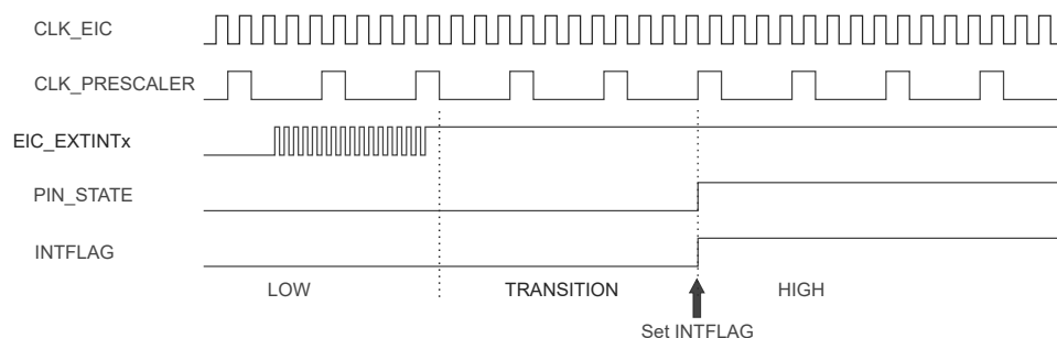
Figure 32-3. EIC_EXTINTx Pin Synchronous Debouncing (Rising Edge)
