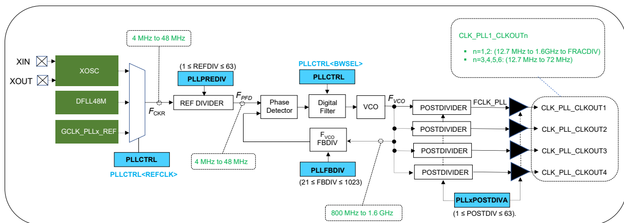
Figure 21-2. PLL Block Diagram
