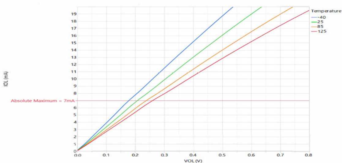
Figure 48-8. IOL vs VOL, 4x Drive Strength I/O on Typical Parts with VDDIO = 3.0V
