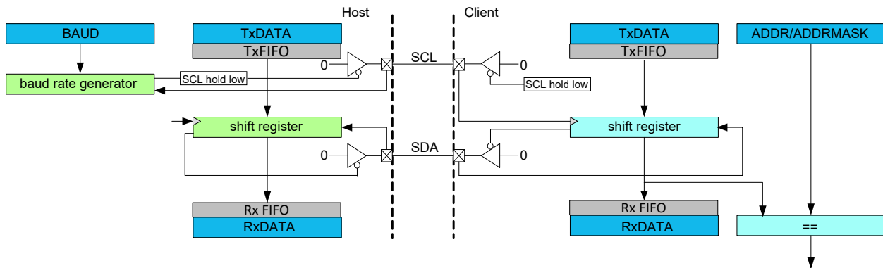
Figure 36-41. I 2 C Single-Host Single-Client Interconnection
