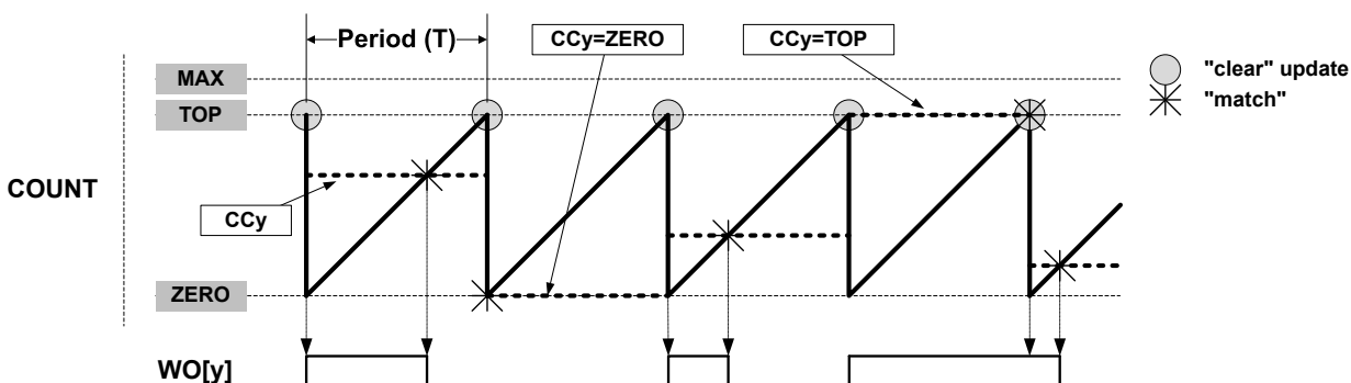
Figure 42-5. Single-Slope PWM Operation
