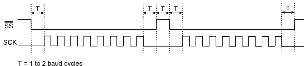
Figure 36-31. Hardware Controlled \overline{SS}
