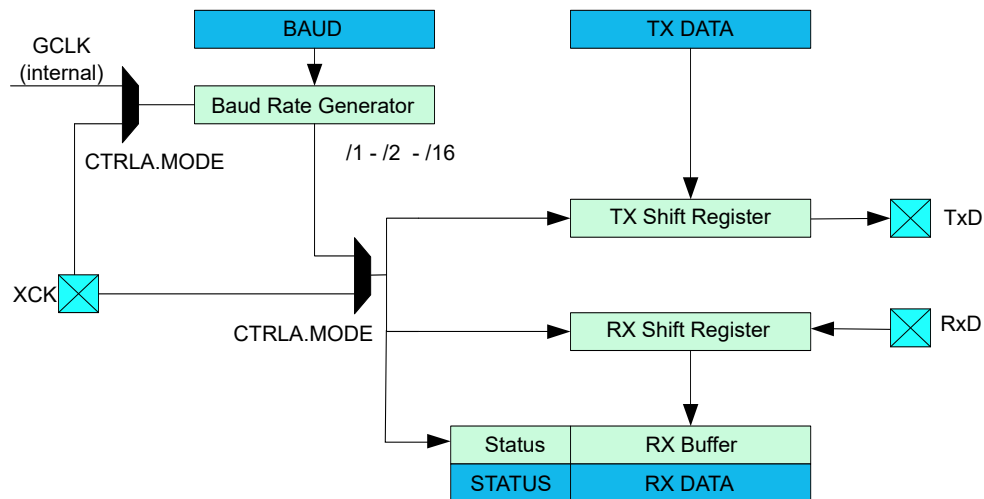
Figure 36-7. USART Block Diagram
