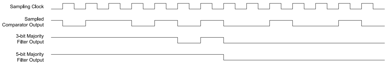
Figure 41-7. Single-Shot Filtering
