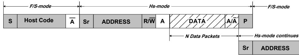
Figure 36-48. High Speed Transfer
