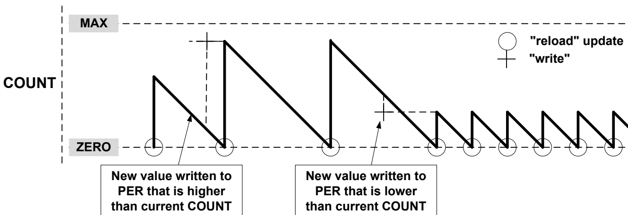
Figure 42-11. Unbuffered Single-Slope Down-Counting Operation
