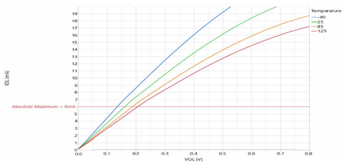
Figure 48-10. IOL vs VOL, 8x Drive Strength I/O on Typical Parts with VDDIO = 3.0V
