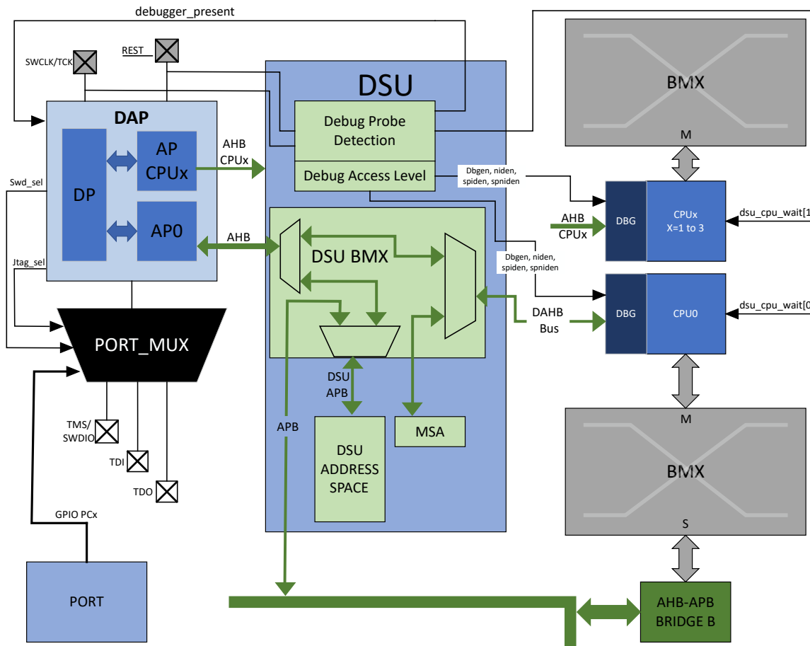
Figure 19-1. Block Diagram
