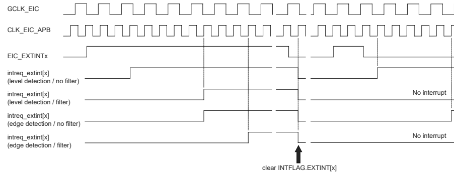
Figure 32-2. Interrupt Detection Latency by Modes (Rising Edge)
