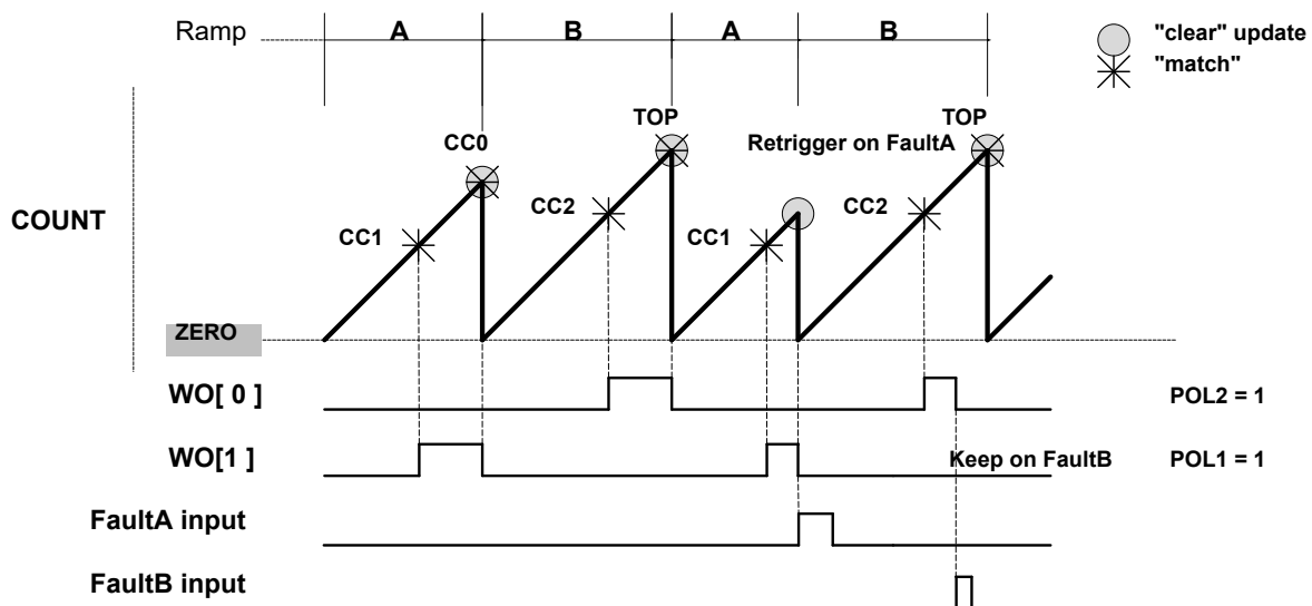
Figure 42-22. RAMP2 Critical Swap Operation
