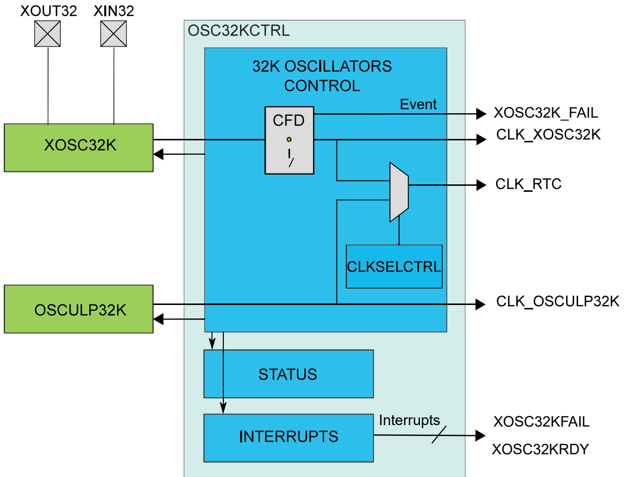
Figure 24-1. OSC32KCTRL Block Diagram
