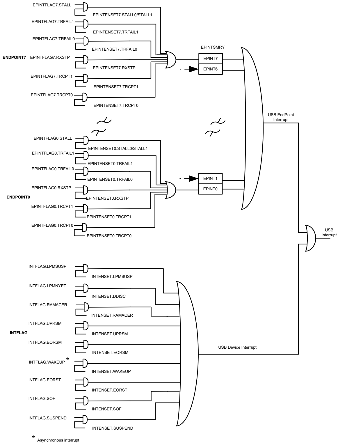
Figure 38-9. Device Interrupt
