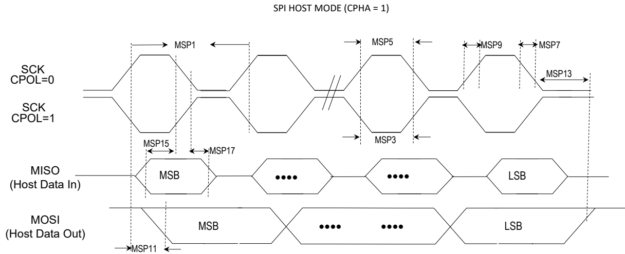
Figure 49-8. SPIx Host Module (CPHA = 1) Timing Diagrams
