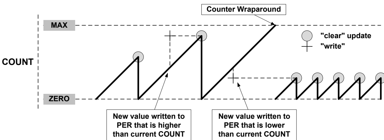
Figure 42-10. Unbuffered Single-Slope Up-Counting Operation
