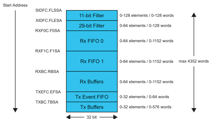
Figure 37-12. Message RAM Configuration
