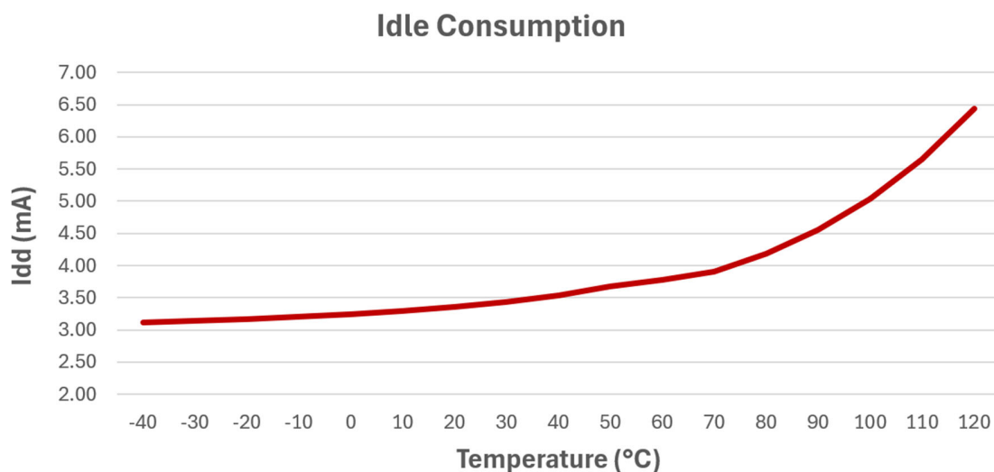
Figure 48-2. Power Consumption over Temperature in Idle mode (Typical values for guidance only, not characterized over process or voltage).
