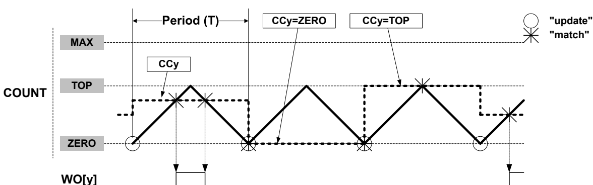
Figure 42-6. Dual-Slope Pulse Width Modulation
