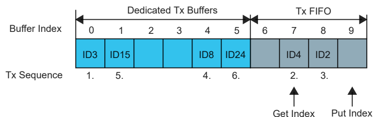
Figure 37-10. Example of mixed Configuration Dedicated Tx Buffers/Tx FIFO
