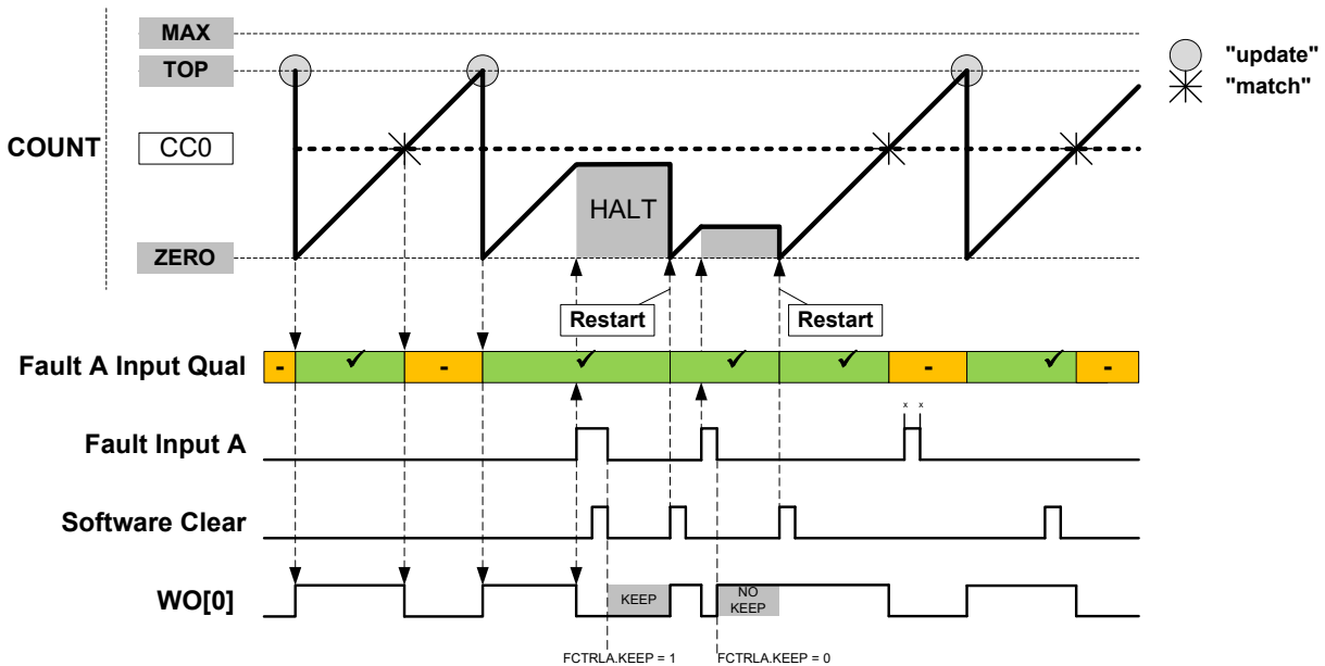
Figure 42-33. Waveform Generation with Software Halt, Fault Qualification, Keep and Restart Actions
