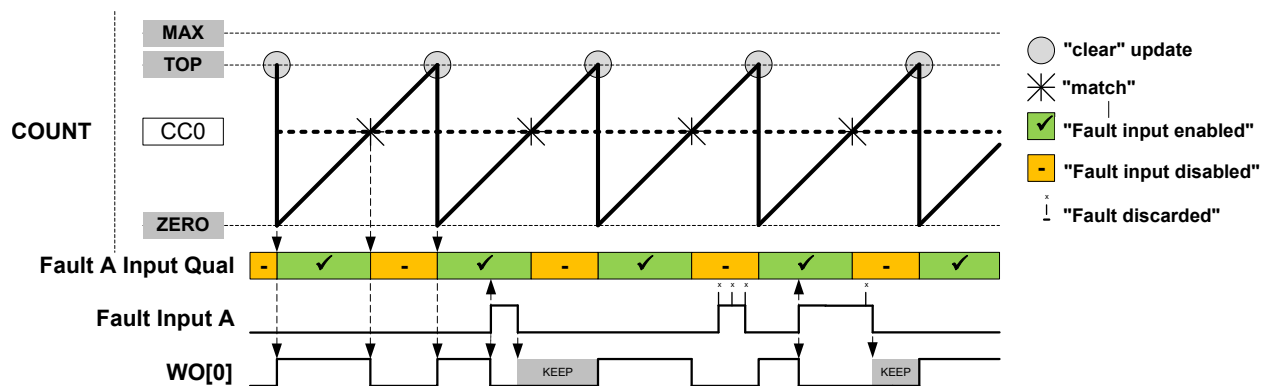
Figure 42-26. Waveform Generation with Fault Qualification and Keep Action
