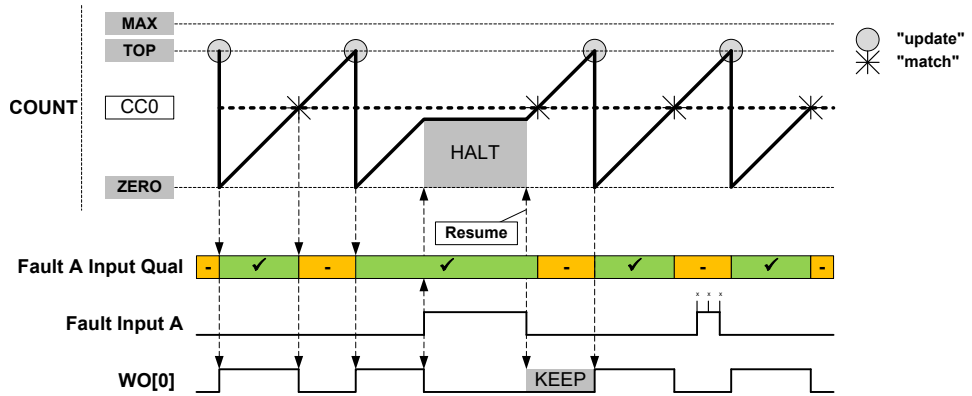
Figure 42-32. Waveform Generation with Fault Qualification, Halt, and Restart Actions
