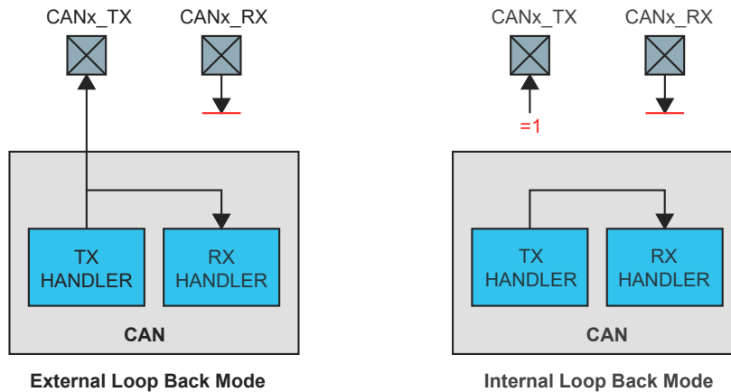
Figure 37-4. Pin Control in Loop-Back Modes
