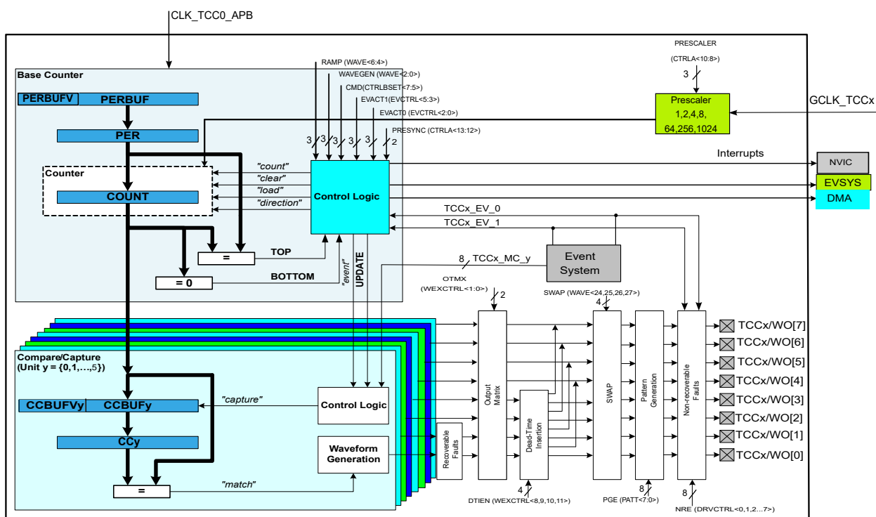
Figure 42-1. Timer/Counter for Control Applications Block Diagram
