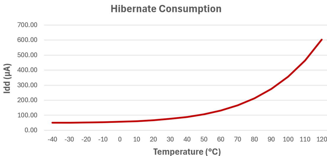
Figure 48-4. Power Consumption over Temperature in Hibernate Mode (Typical values for guidance only, not tested)
