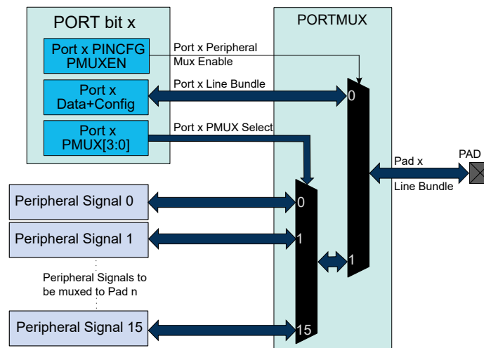
Figure 35-3. Overview of the Peripheral Functions Multiplexing
