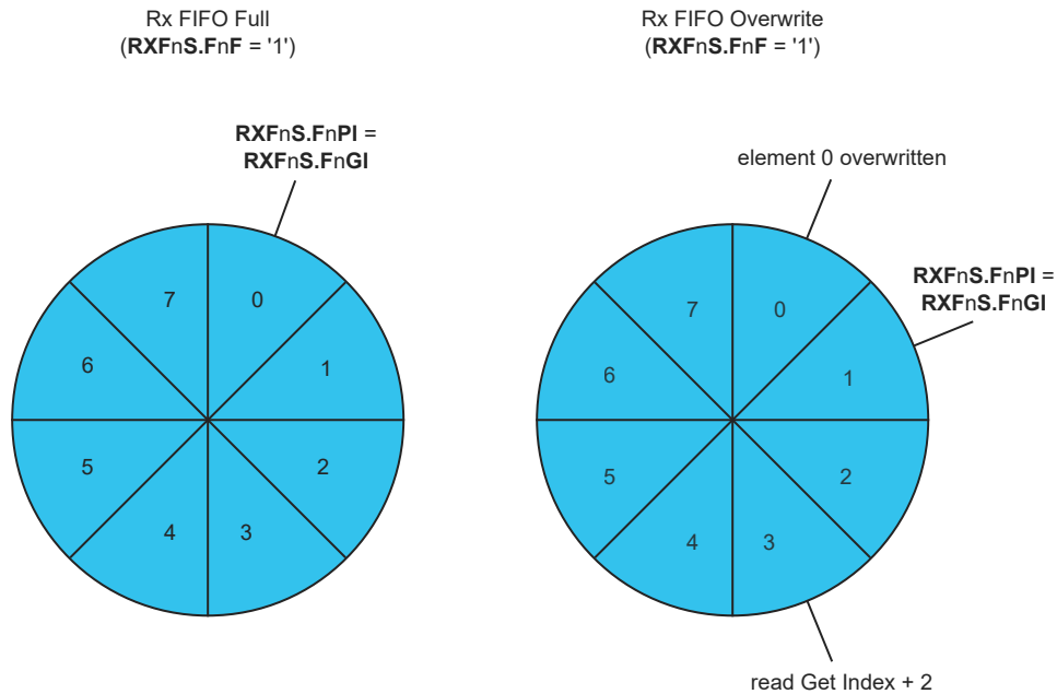
Figure 37-8. Rx FIFO Overflow Handling (n = 0 for Rx FIFO 0 buffer and n = 1 for Rx FIFO 1 buffer)
