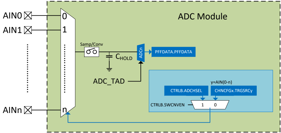
Figure 40-1. ADC Block Diagram
