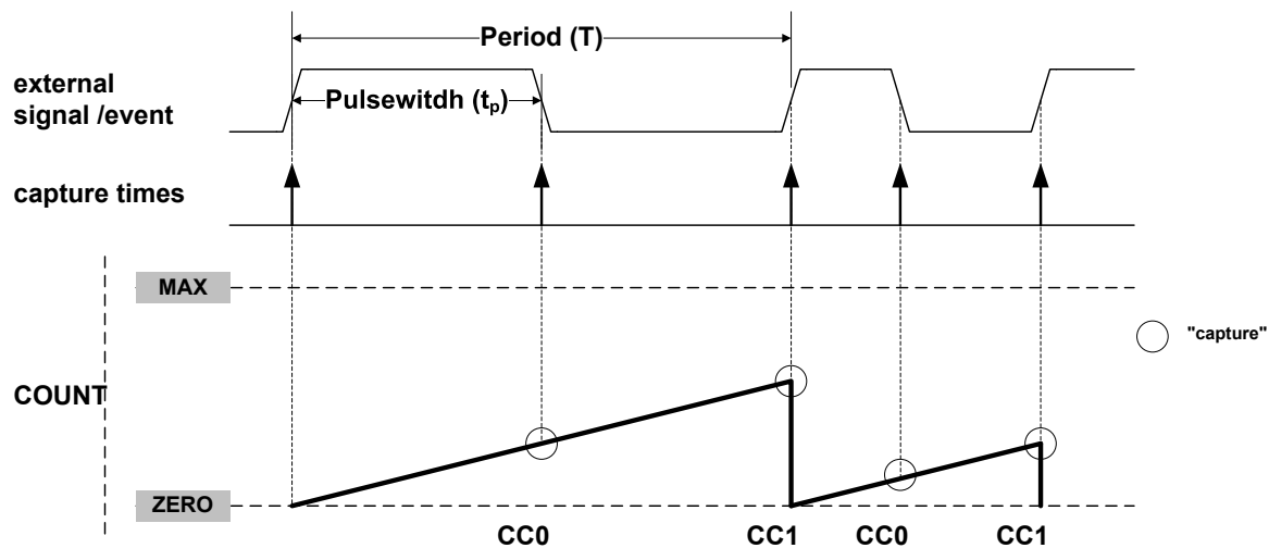
Figure 42-16. PWP Capture
