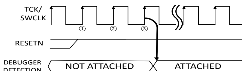
Figure 19-3. Hot-Plugging Detection Timing Diagram
