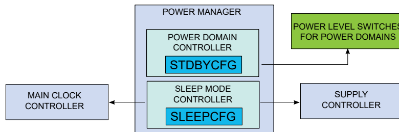
Figure 30-1. Power Manager Block Diagram
