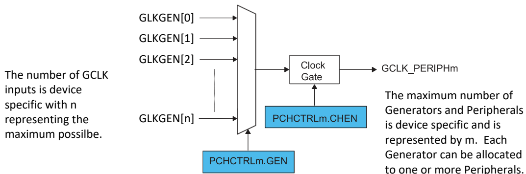
Figure 22-4. Peripheral Clock
