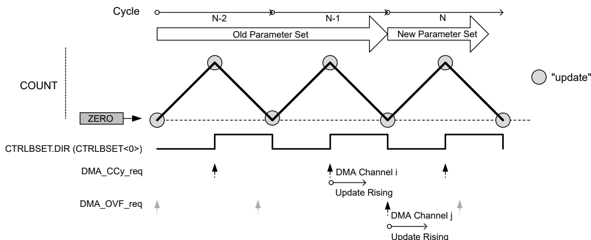
Figure 42-36. DMA Triggers in DSBOOTH Operation and Circular Buffer Enabled
