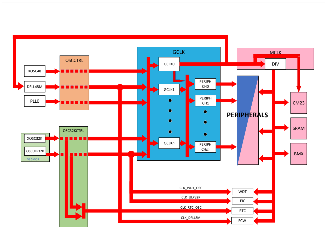
Figure 20-1. Clock Distribution Block Diagram
