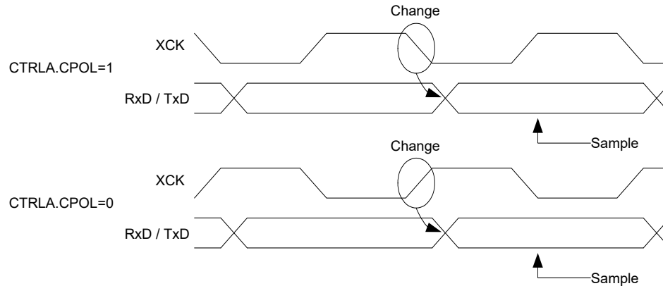
Figure 36-10. Synchronous Mode XCK Timing
