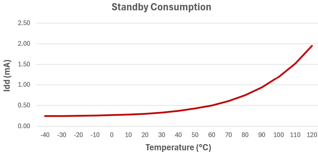
Figure 48-3. Power Consumption over Temperature in Standby Mode (Typical values for guidance only, not tested)
