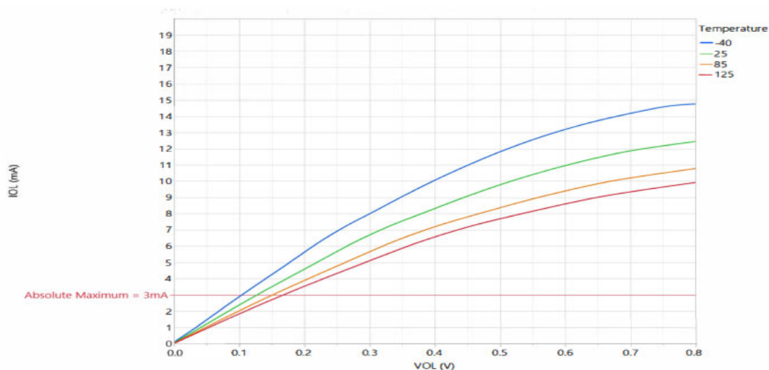
Figure 48-7. IOL vs VOL, 4x Drive Strength I/O on Typical Parts with VDDIO = 1.71V
