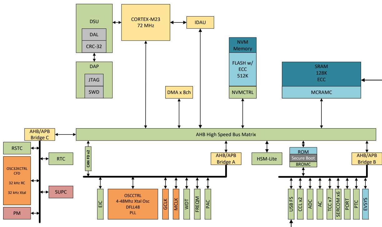
Figure 4-1. PIC32CM SG00 Block Diagram
