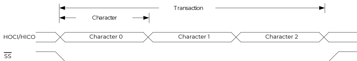
Figure 36-26. SPI Transaction Format
