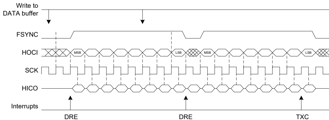
Figure 36-38. FMODE = HOST, FSPOL = HIGH, FSLEN = LEVEL, FSES = 1
