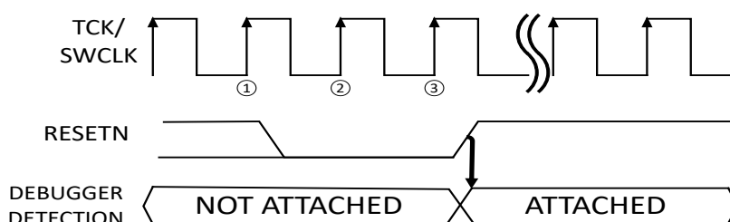
Figure 19-2. Cold-Plugging Timing Diagram
