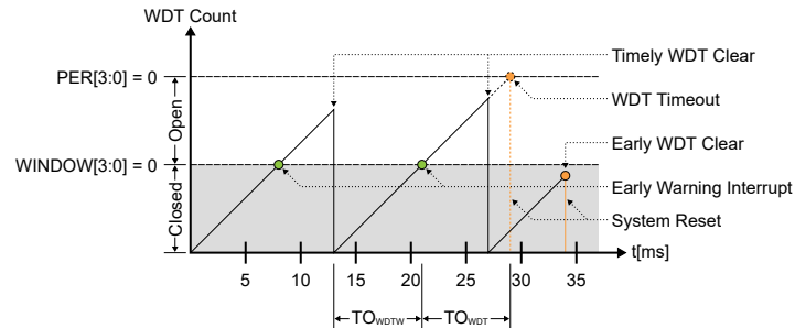
Figure 25-3. Window-Mode Operation
