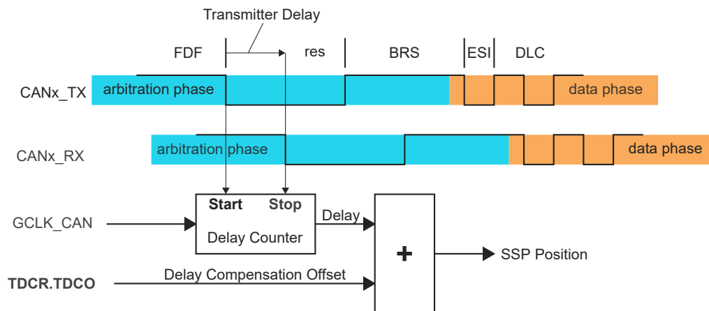
Figure 37-2. Transceiver delay measurement
