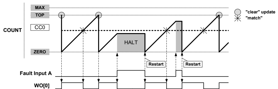
Figure 42-31. Waveform Generation with Halt and Restart Actions
