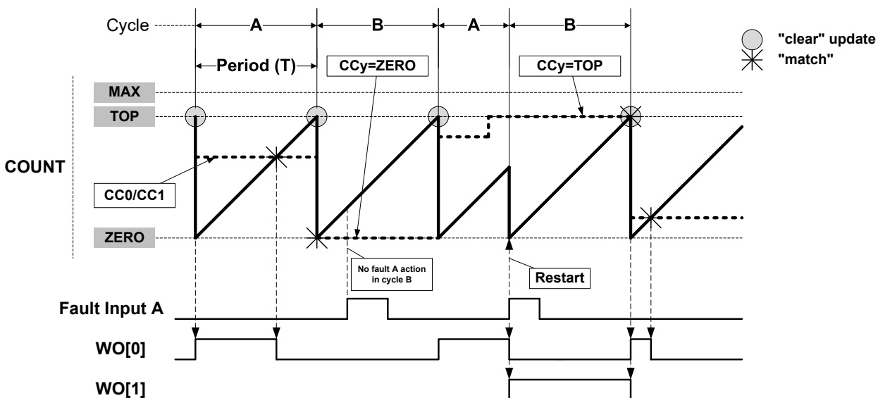
Figure 42-28. Waveform Generation in RAMP2 Operation with Restart Action
