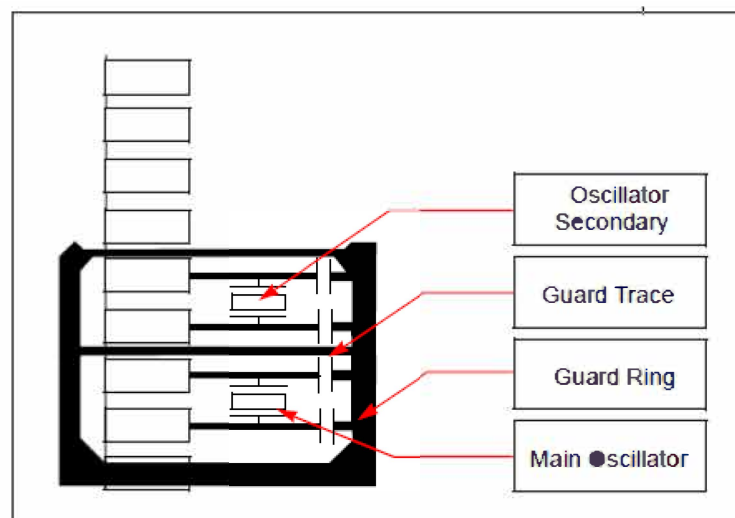
Figure 1-1. Suggested Oscillator Circuit Placement
