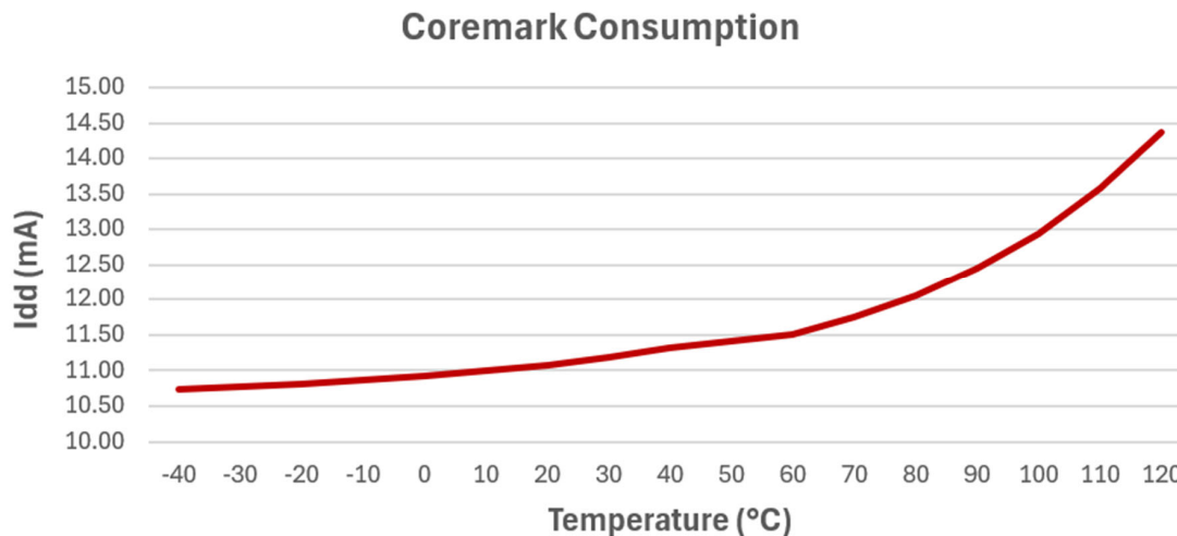
Figure 49-1. Power Consumption over Temperature in Active Mode (Typical values for guidance only, not tested)
