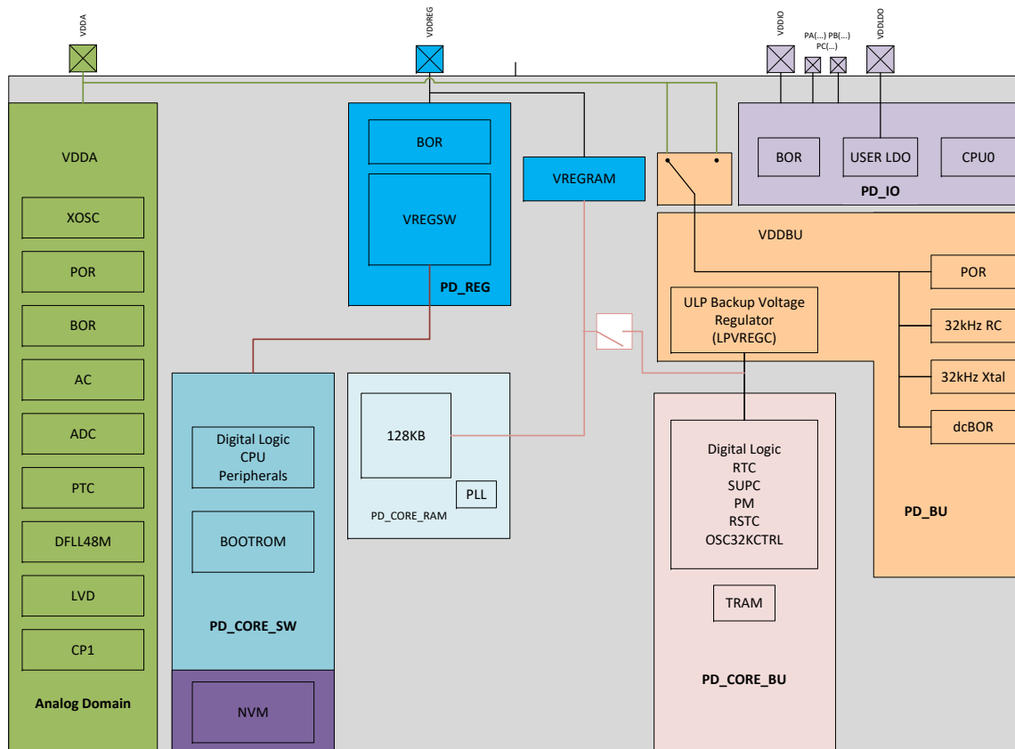
Figure 8-1. Power Domain Block Diagram
