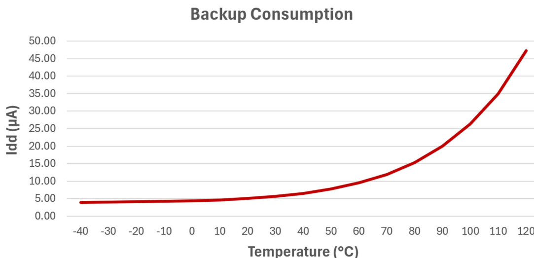
Figure 48-5. Power Consumption over Temperature in Backup Mode (Typical values for guidance only, not tested)
