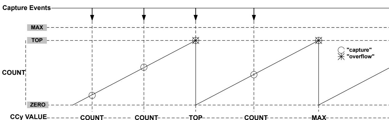
Figure 42-34. Time-Stamp
