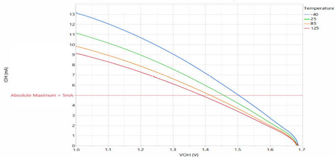
Figure 48-11. IOH vs VOH, 4x Drive Strength I/O on Typical Parts with VDDIO = 1.71V
