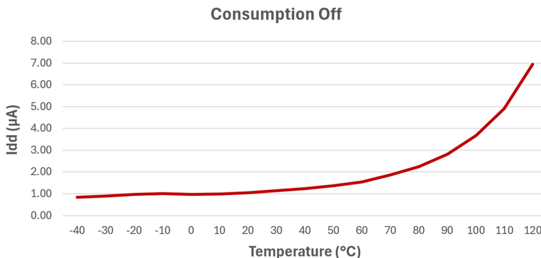
Figure 48-6. Power Consumption over Temperature in Off Mode (Typical values for guidance only, not tested)
