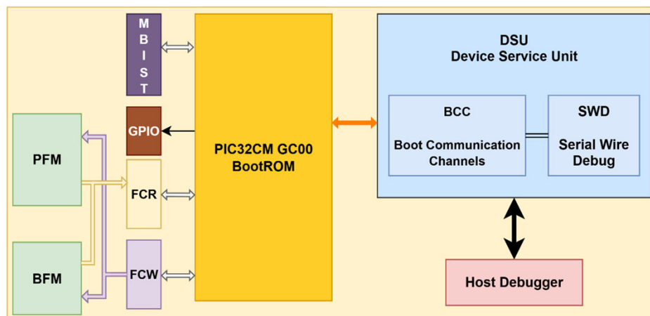
Figure 16-1. PIC32 GC00 Boot ROM Block Diagram
