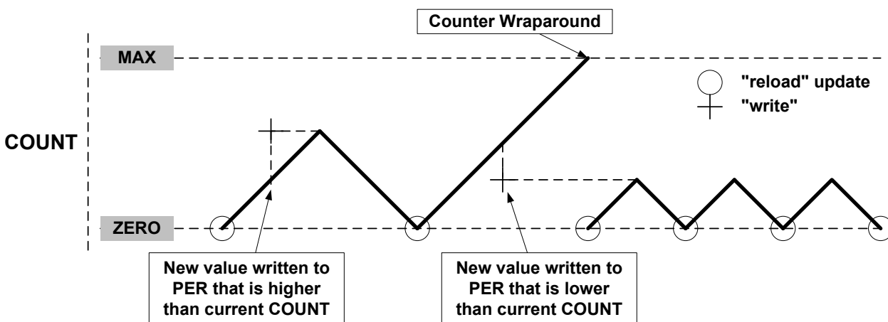
Figure 42-12. Unbuffered Dual-Slope Operation
