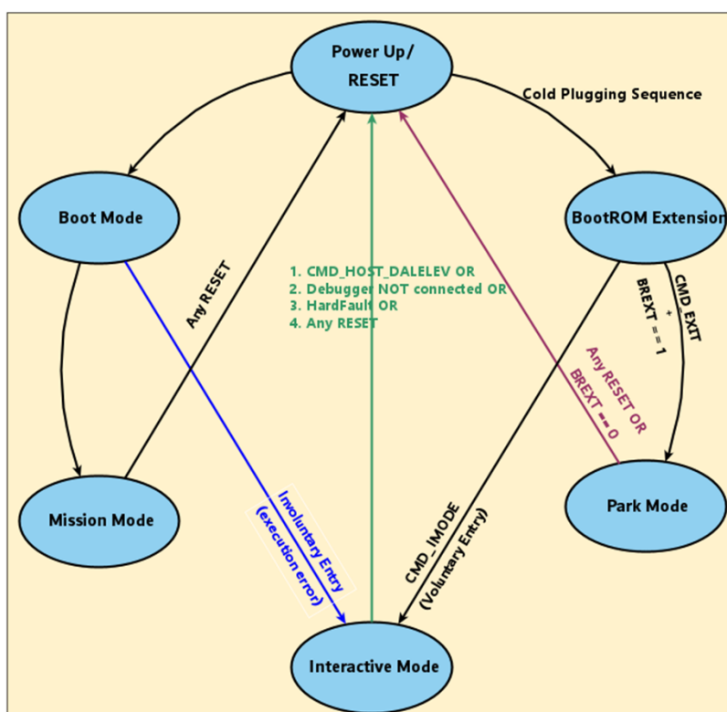
Figure 16-4. Diagram of Modes
