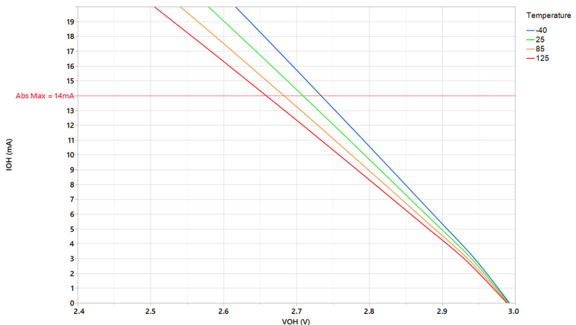
Figure 48-14. IOH vs VOH, 8x Drive Strength I/O on Typical Parts with VDDIO = 3.0V
