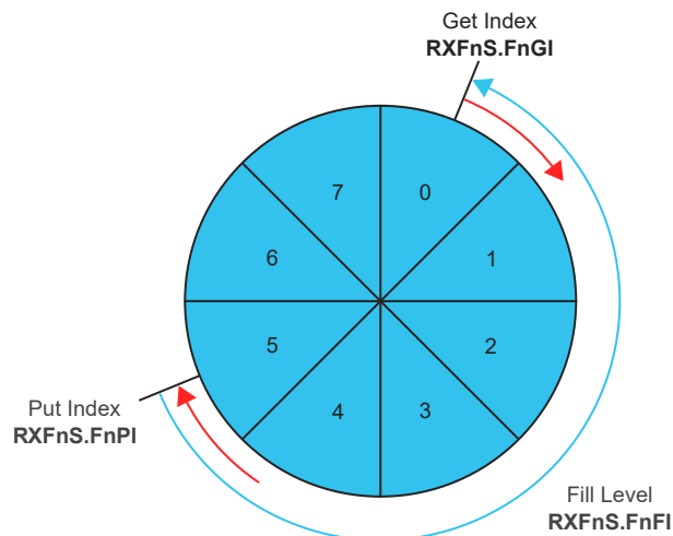
Figure 37-7. Rx FIFO Status (n = 0 for Rx FIFO 0 buffer and n = 1 for Rx FIFO 1 buffer)
