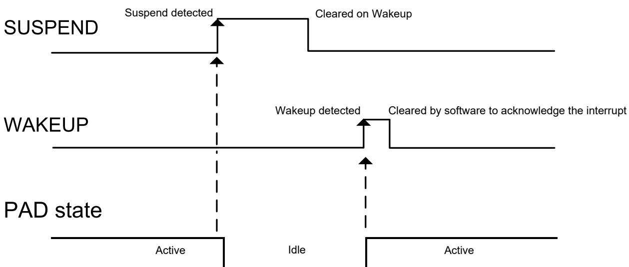
Figure 38-8. Pad Events
