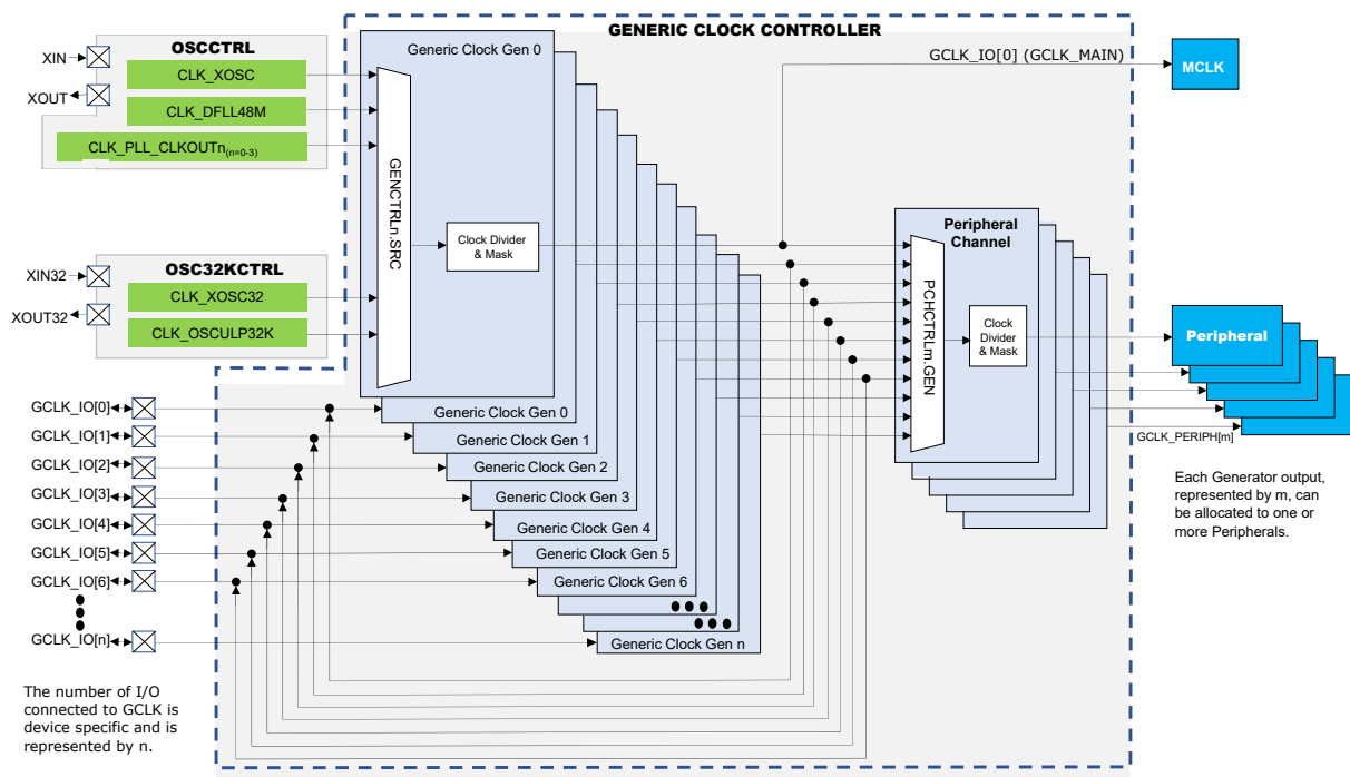
Figure 22-1. Device Clocking Diagram
