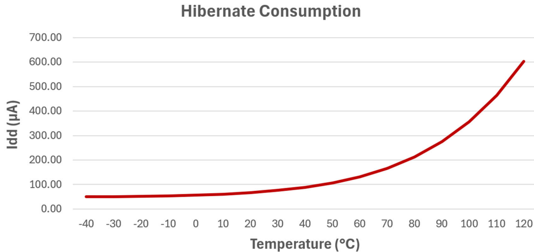
Figure 49-4. Power Consumption over Temperature in Hibernate Mode (Typical values for guidance only, not tested)
