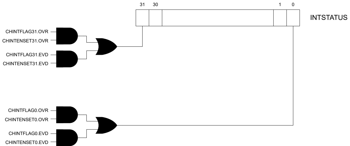
Figure 34-2. Interrupt Status Register
