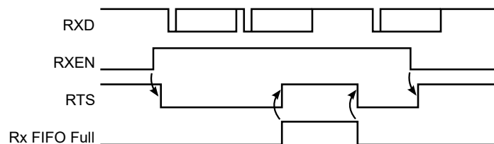
Figure 36-14. Receiver Behavior when Operating with Hardware Handshaking
