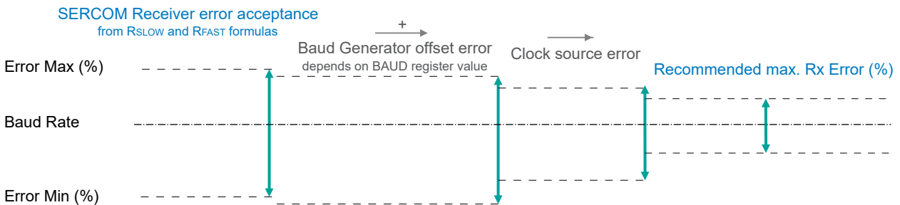
Figure 36-11. USART Rx Error Calculation
