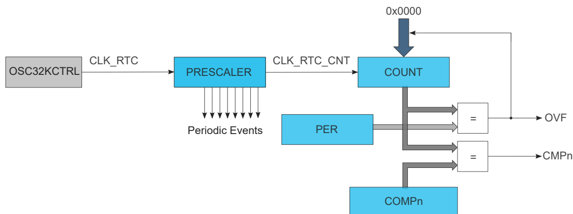
Figure 27-2. RTC Block Diagram (Mode 1 — 16-Bit Counter)
