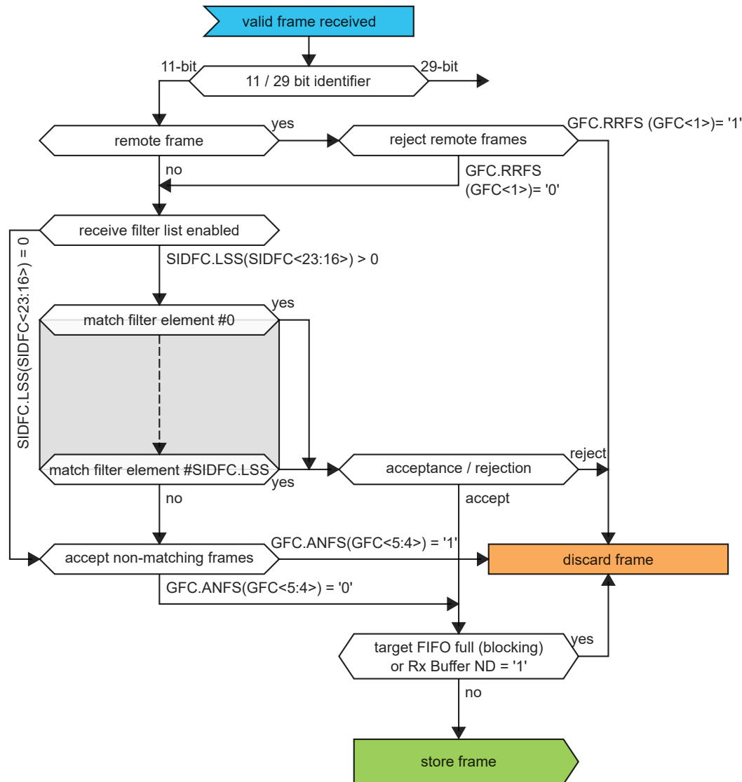
Figure 37-5. Standard Message ID Filtering
