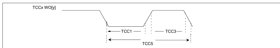
Figure 49-12. TCCx Timer Compare Output Module AC Timing Diagrams
