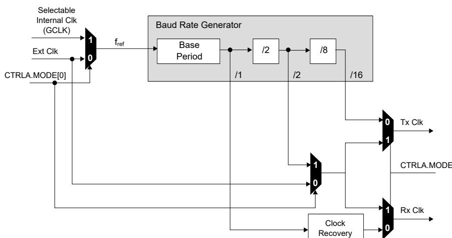
Figure 36-3. Baud Rate Generator
