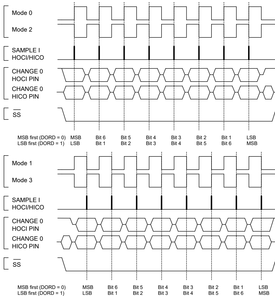
Figure 36-27. SPI Transfer Modes
