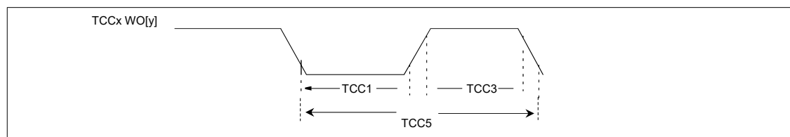
Figure 48-26. TCCx Timer Capture Input Module AC Timing Diagrams
