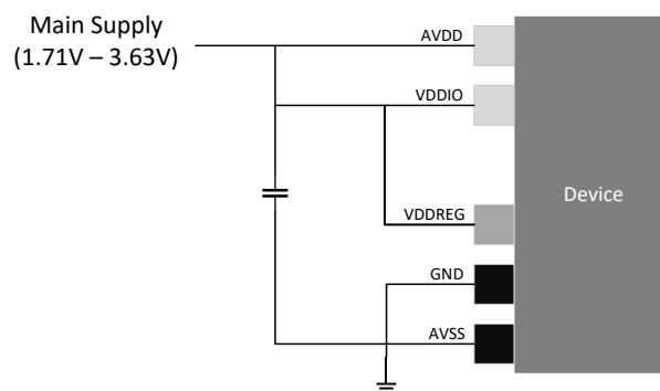
Figure 8-2. Power Supply Connection for Single Voltage Mode
