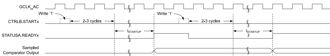
Figure 41-3. Single-Shot Example
