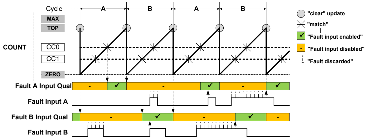
Figure 42-25. Fault Qualification in RAMP2 Operation with Inverted Polarity
