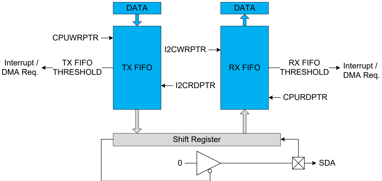
Figure 36-57. FIFO Overview
