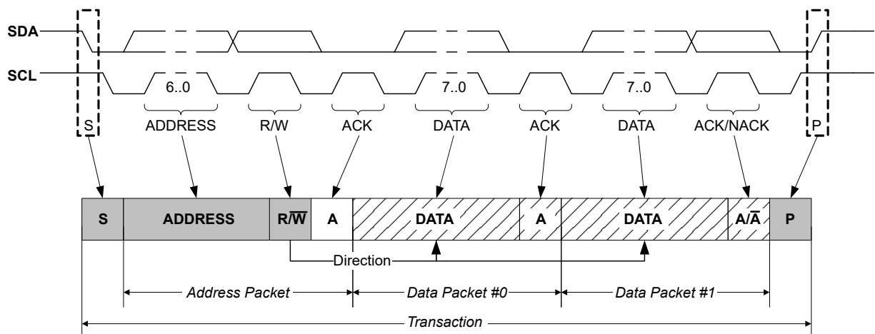
Figure 36-43. Basic I 2 C Transaction Diagram
