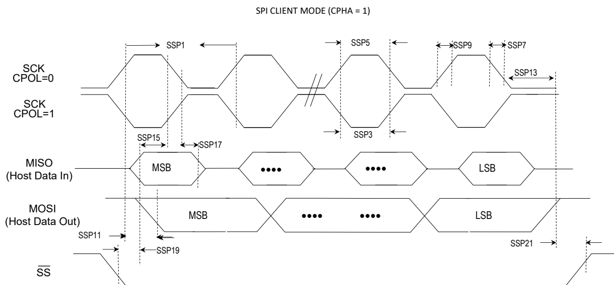
Figure 48-20. SPIx Client Module (CPHA = 1) Timing Diagrams
