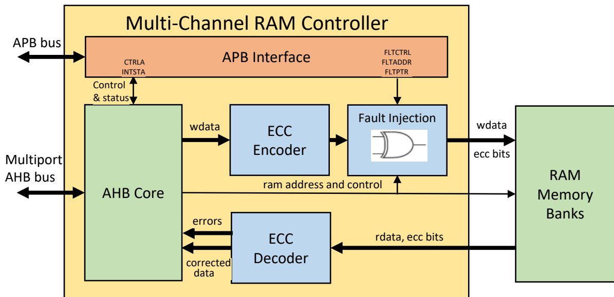
Figure 17-1. MCRAMC Block Diagram
