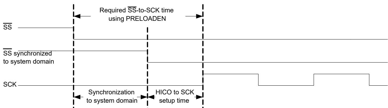
Figure 36-28. Timing Using Preloading
