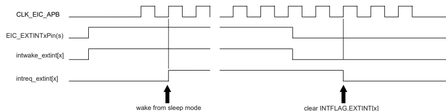
Figure 32-5. Wake-up Operation Example (High-Level Detection, No Filter, Interrupt Enable Set)
