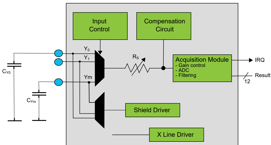
Figure 44-2. PTC Block Diagram Self Capacitance
