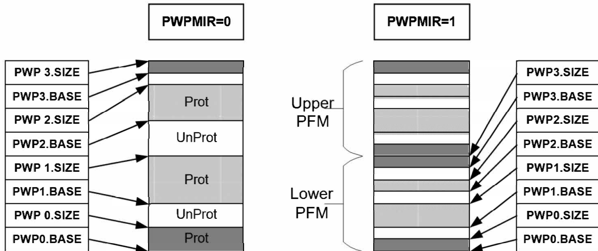
Figure 33-2. PWP Example: No Mirror versus Mirror
