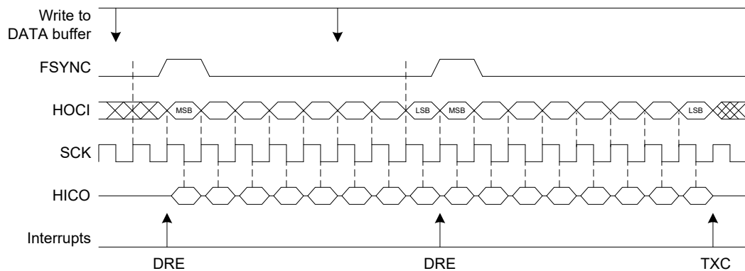
Figure 36-37. FMODE = HOST, FSPOL = HIGH, FSLEN = STROBE, FSES = 1
