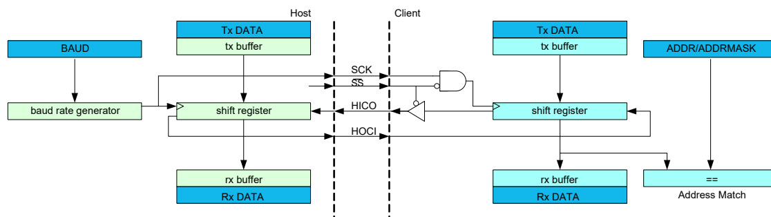
Figure 36-25. Full-Duplex SPI Host Client Interconnection
