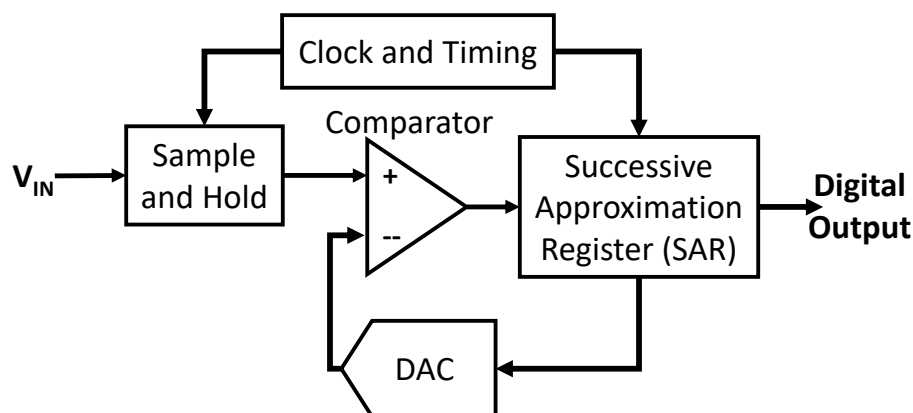
Figure 40-3. ADC Module Architecture
