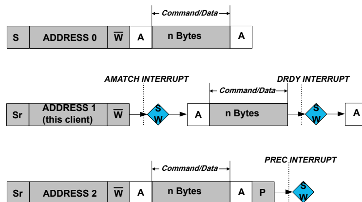
Figure 36-53. PMBus Group Command Example
