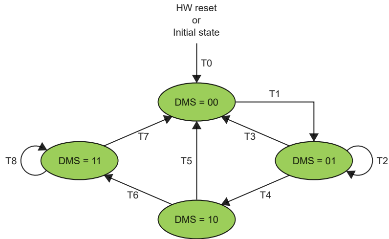
Figure 37-9. Debug Message Handling State Machine
