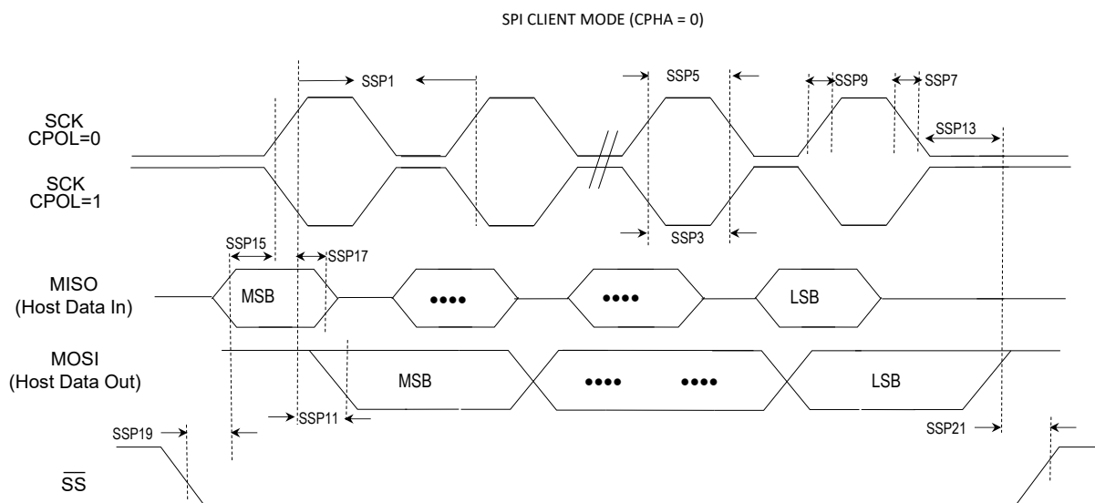
Figure 49-9. SPIx Client Module (CPHA = 0) Timing Diagrams
