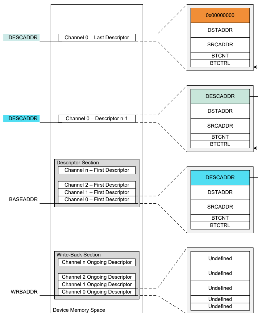
Figure 28-3. Memory Sections
