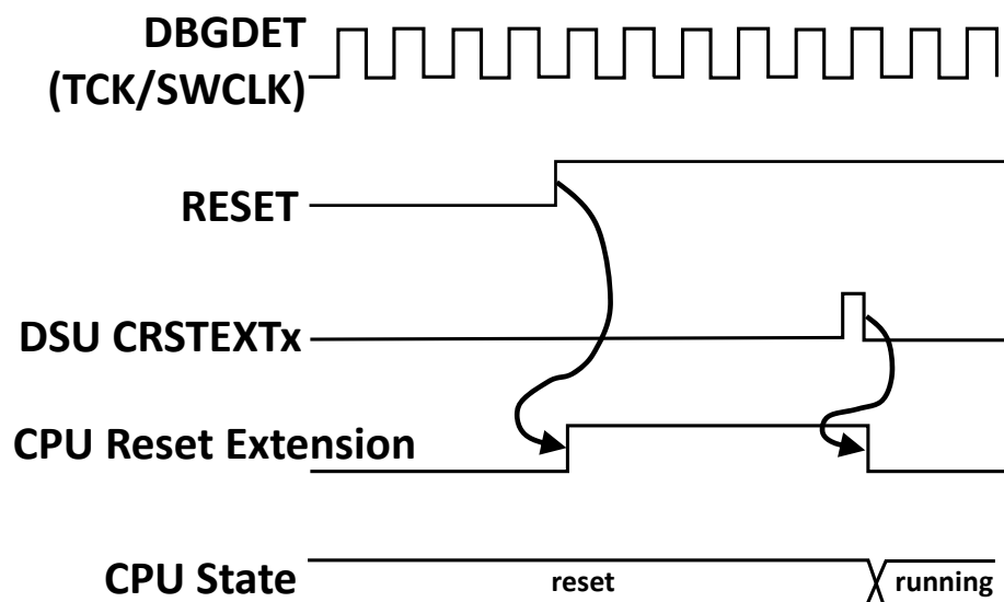
Figure 19-4. Typical CPU Reset Extension Set and Clear Timing Diagram
