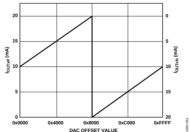
Figure 48. DAC Output Currents vs. DAC Offset Value
