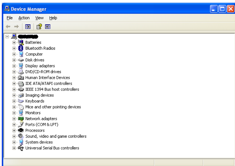
Figure 2.8 - Device Manager
