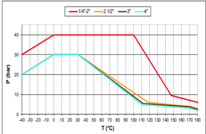
PRESSURE-TEMPERATURE CHART
