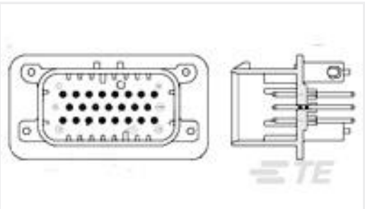
TE Part #1-776231-1 35POS, PIN DIA 1.3, HDR ASSY, 180DEG, COD 1
