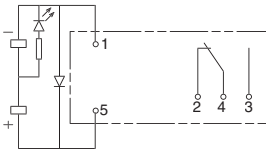
G2R-1-SND, G2R-1-SNDI (c.c.)
