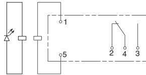
G2R-1-SND, G2R-1-SNDI (c.c.)
