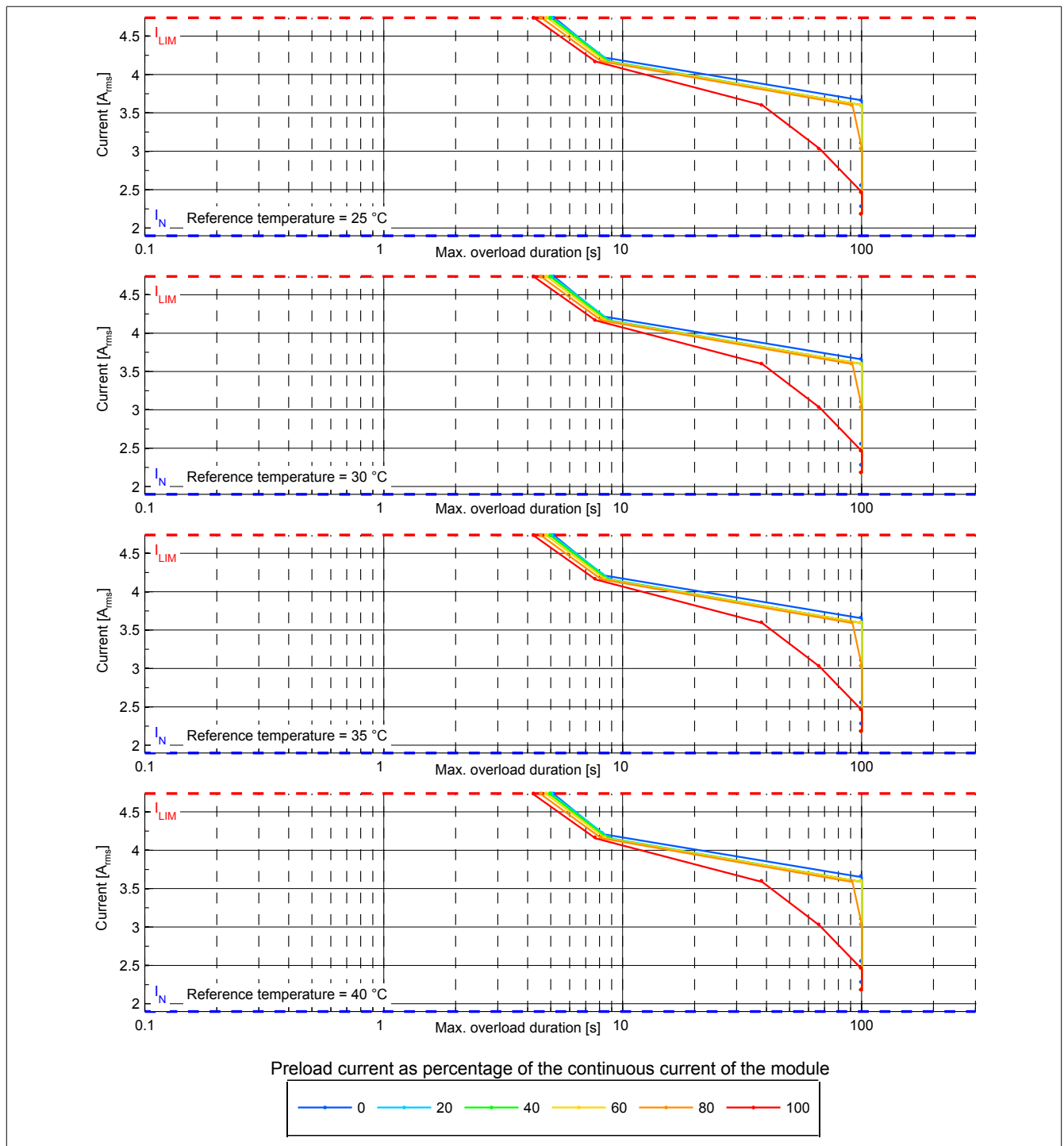
Figure 2: 8BVI0014HWSSx.000-x - Overload characteristics, overload response - ERROR+STOP
