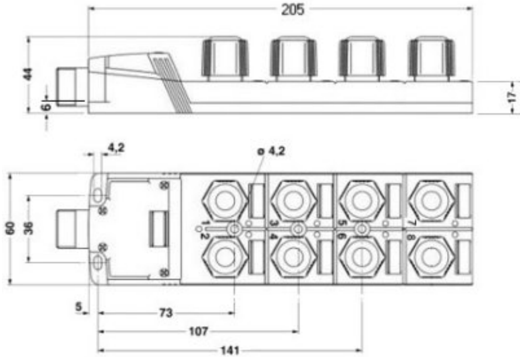
Dimensioned drawing
