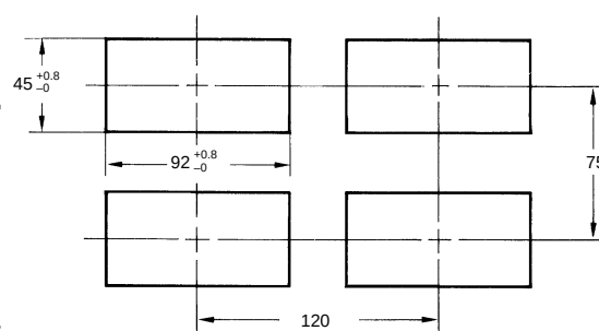
Panel Cutouts
