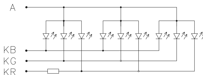
CIRCUIT DIAGRAM
