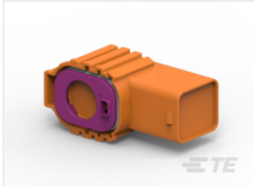
TE Part # 2137704-2 HV1100 1POS PLUG HSG ASSY SLD 90 DEG
