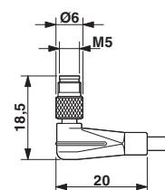
Dimensioned drawing
