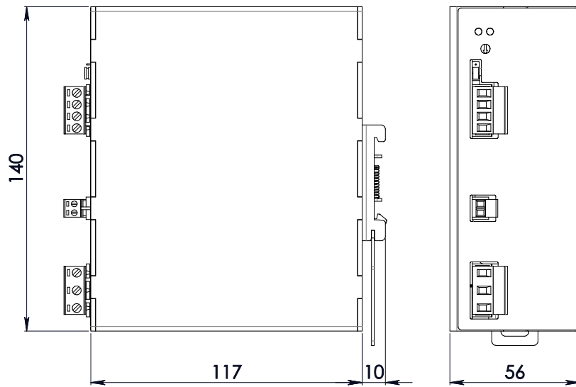
Figure 1. Mechanical Drawing
