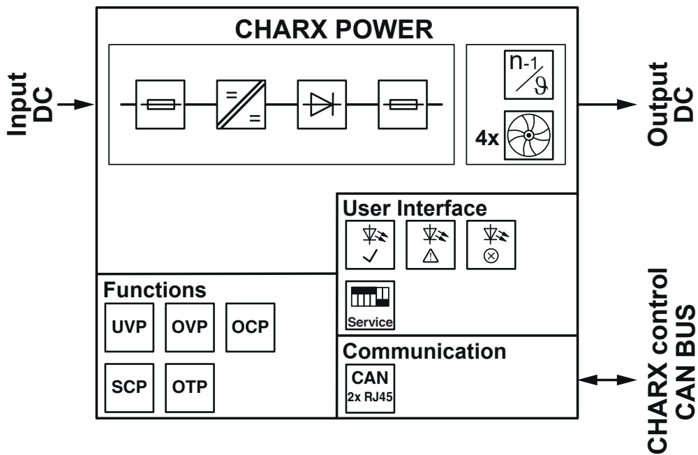
Block diagram
