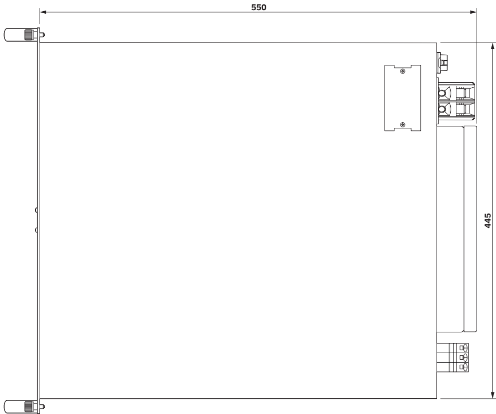
Dimensional drawing
