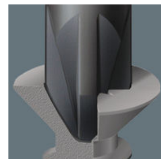
The Wera Black Point tip and a refined hardening process ensure long service life of the tip, improved corrosion protection and an exact fit.
