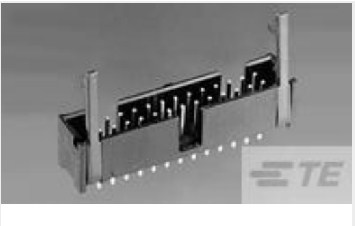
TE Part #2-1761712-7 IDC LOW PRO HDR 20P RA LAT
