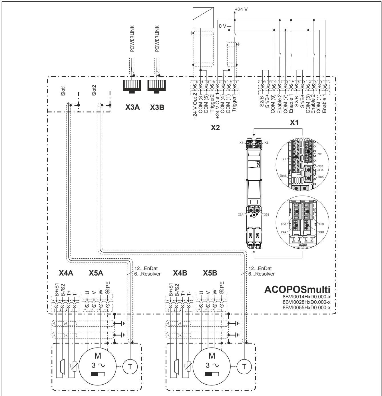
Figure 6: 8BVI0014HxD0.000-x, 8BVI0028HxD0.000-x, 8BVI0055HxD0.000-x - Pinout overview
