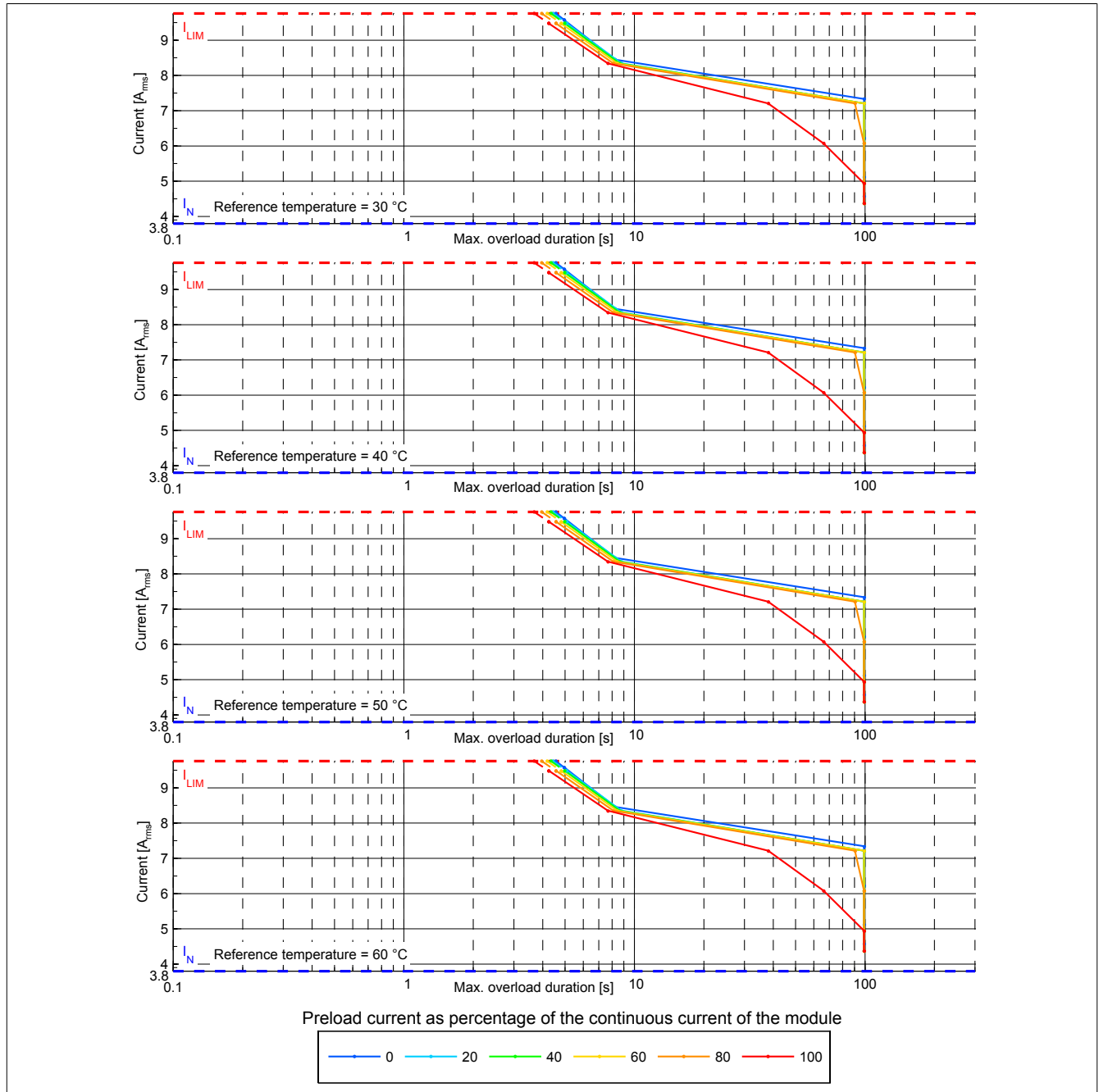
Figure 1: 8BVI0028HCDx.000-x - Overload characteristics, overload response - WARNING
