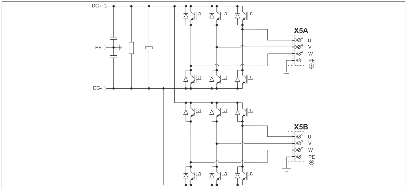
Figure 10: Motor
