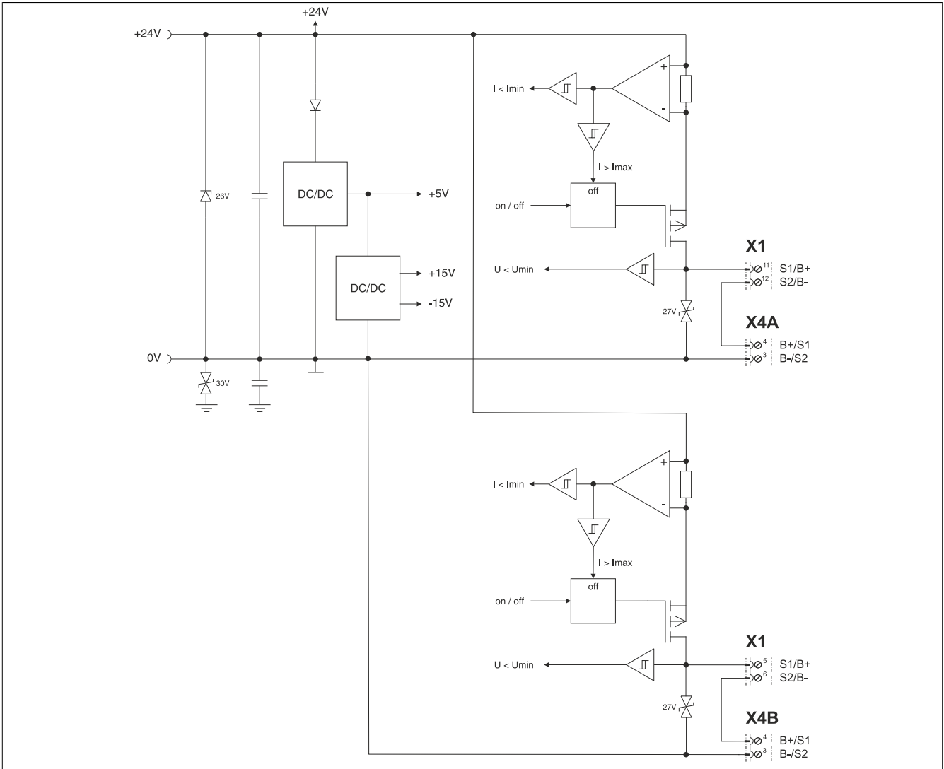
Figure 8: Holding brake
