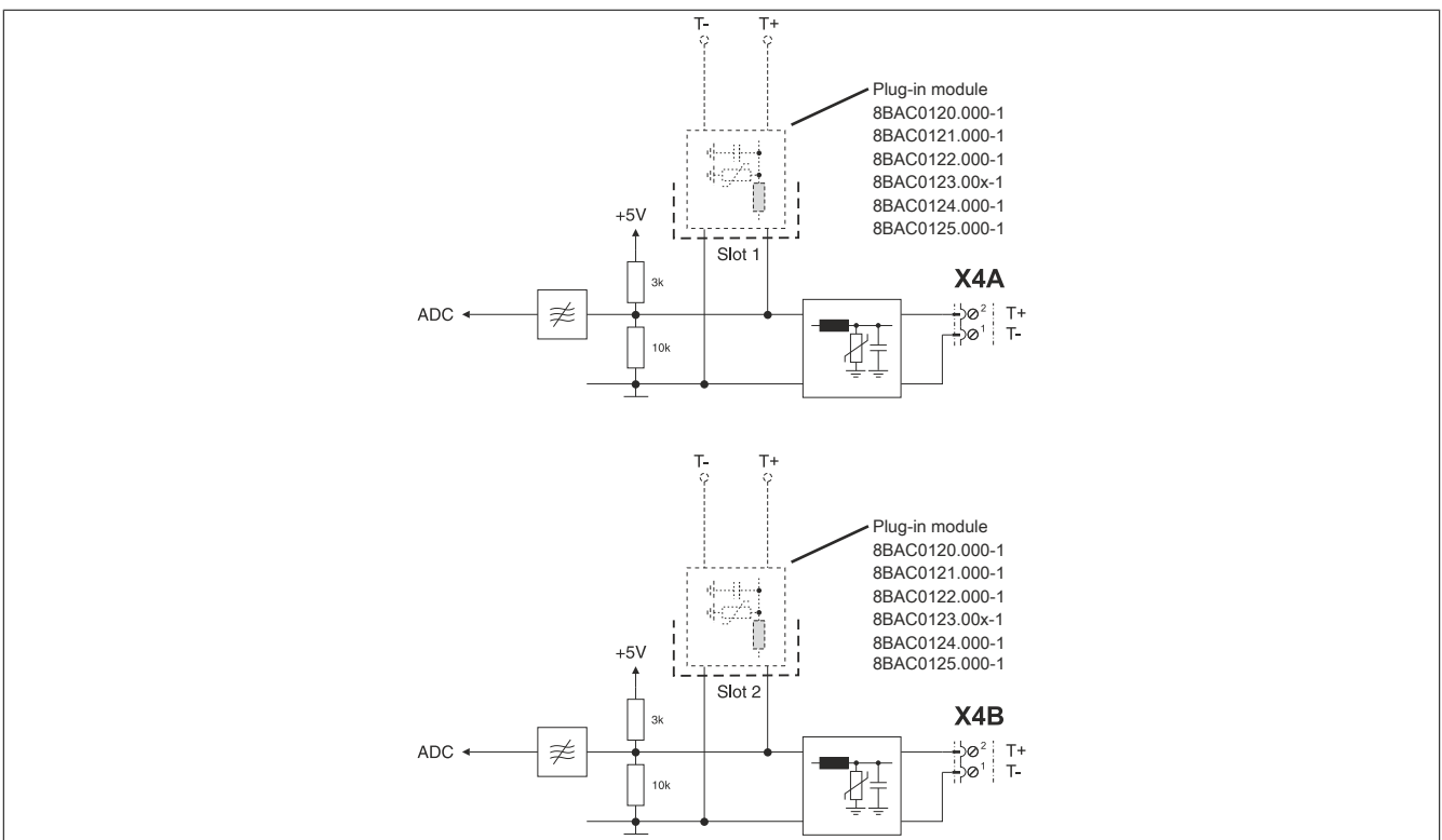
Figure 9: Temperature sensor
