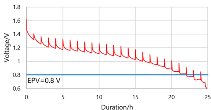
Toy[2.2Ω 1h/day]
