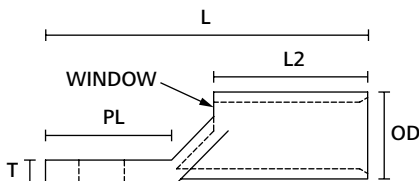
Copper Lug Series, Side View
