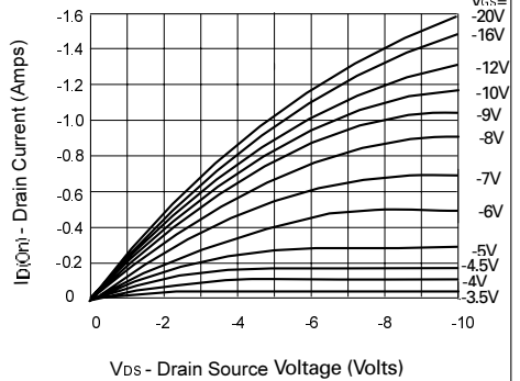
Saturation Characteristics
