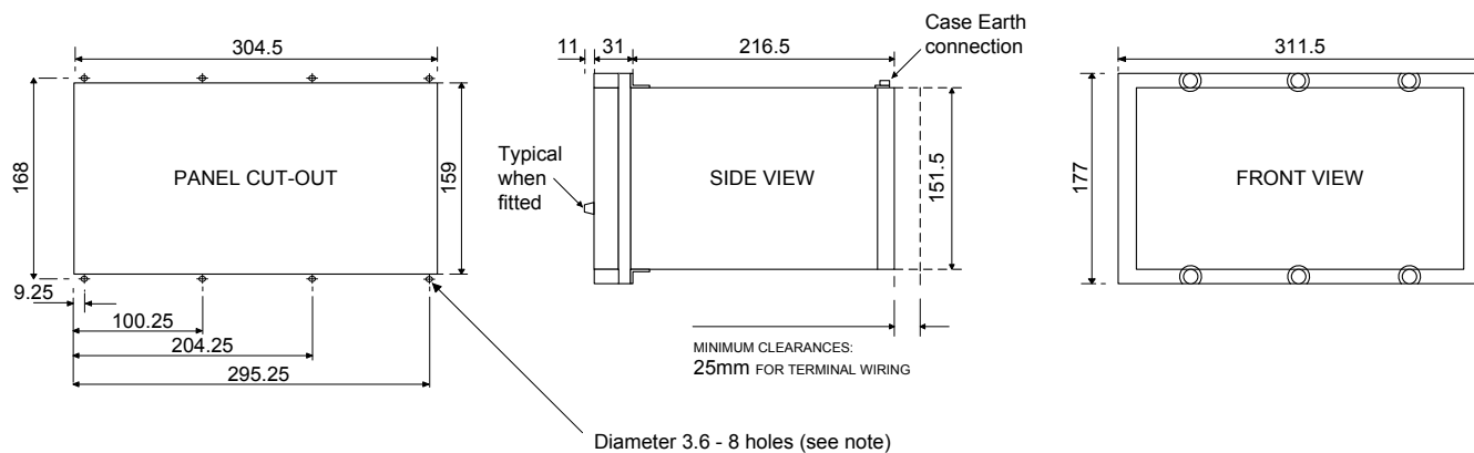
Fig 11. E12 Case (4U high)
