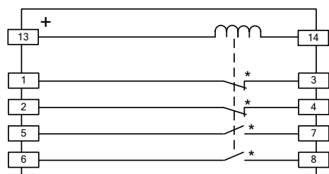
Fig 20. 7PG2183 B34 Delayed Pickup delay relay for Rf Mode Intertipping (E2 case)
