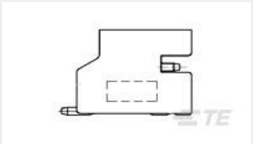
TE Part #1775469-8 HPI CONN., 2.0MM, R/A, SMT, 8P, 80U"
