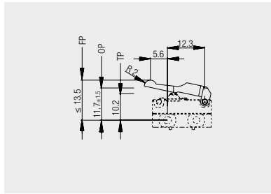
L32: simulated roller, mounted on NC side 190.372.041
