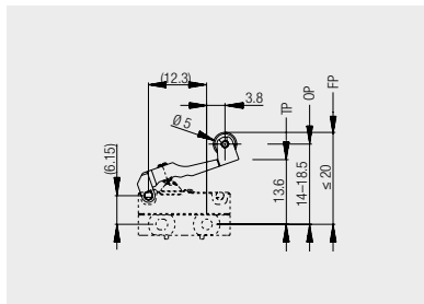
L43: adjustable roller lever 190.072.013
