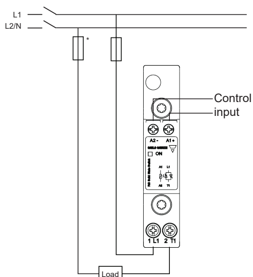
Variant without Over Temperature Protection
