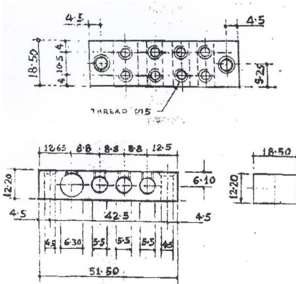
Drawing (mm):
