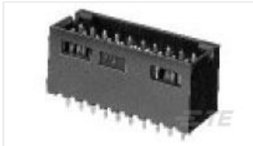
TE Part #6-102618-3 30 MODII HDR DRST SHRD .100CL
