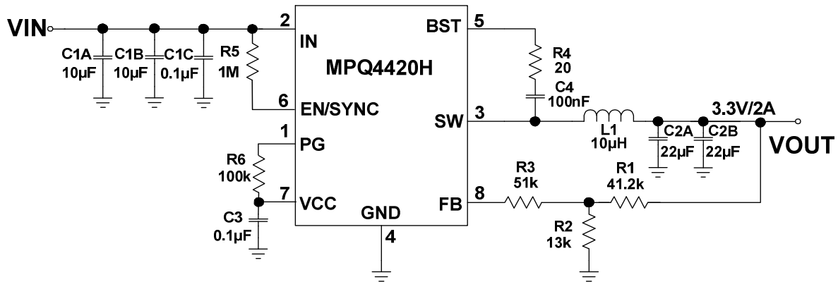
Figure 8: 3.3V Output Typical Application Circuit
