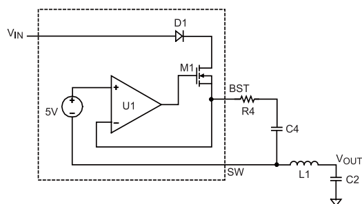
Figure 3: Internal Bootstrap Charging Circuit
