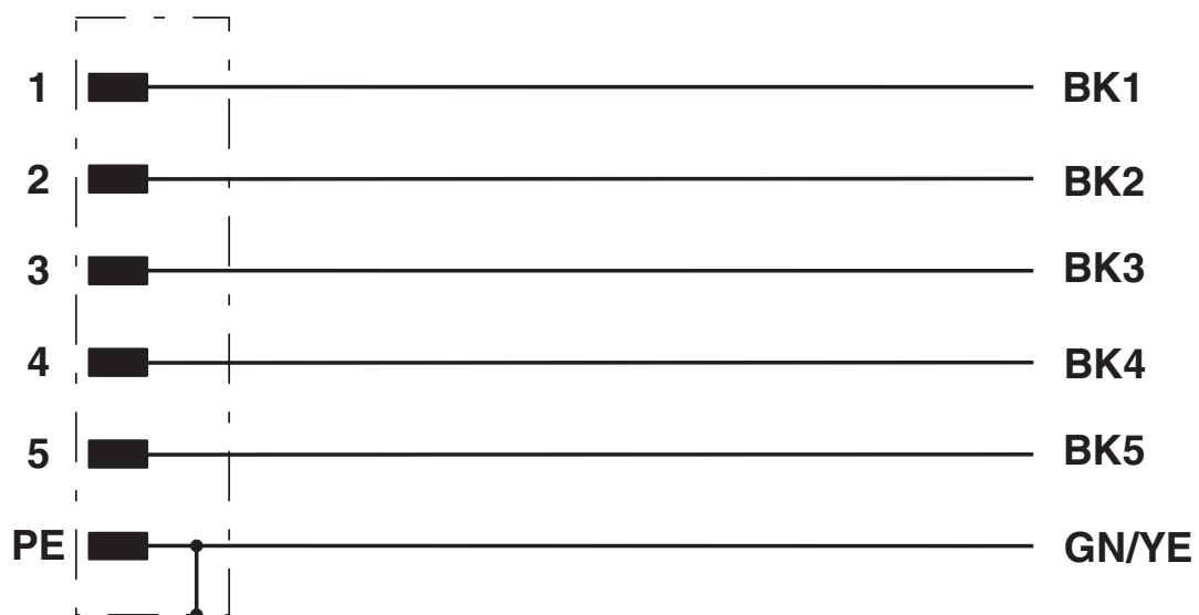
Circuit diagram
