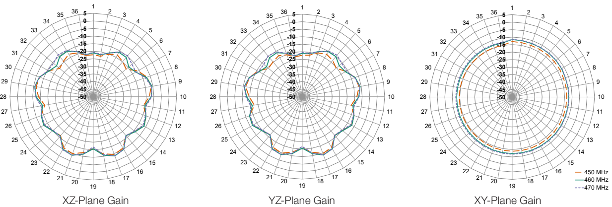
Figure8. Radiation Patterns for ANT-450-RHS-SMA Antenna
