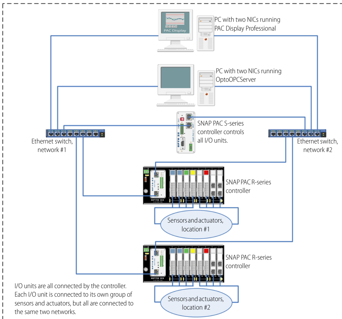
Opto 22 Redundant Network
