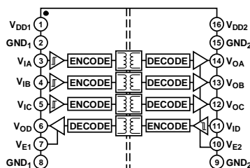
Figure 2. ADuM3401 Functional Block Diagram
