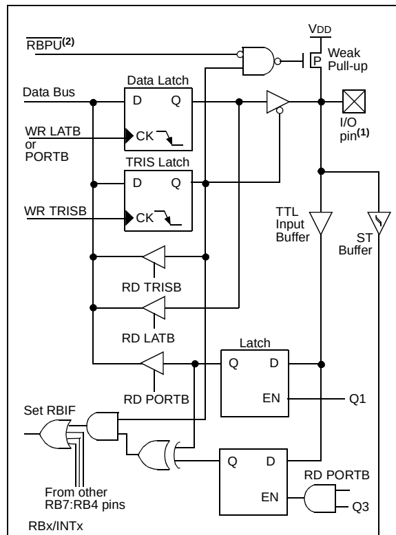
FIGURE 8-4: BLOCK DIAGRAM OF RB7:RB4 PINS
