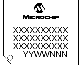
44-Lead TQFP
