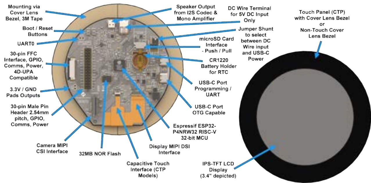
Hardware Layout (3.4" CTP w/ CLB Module depicted)
